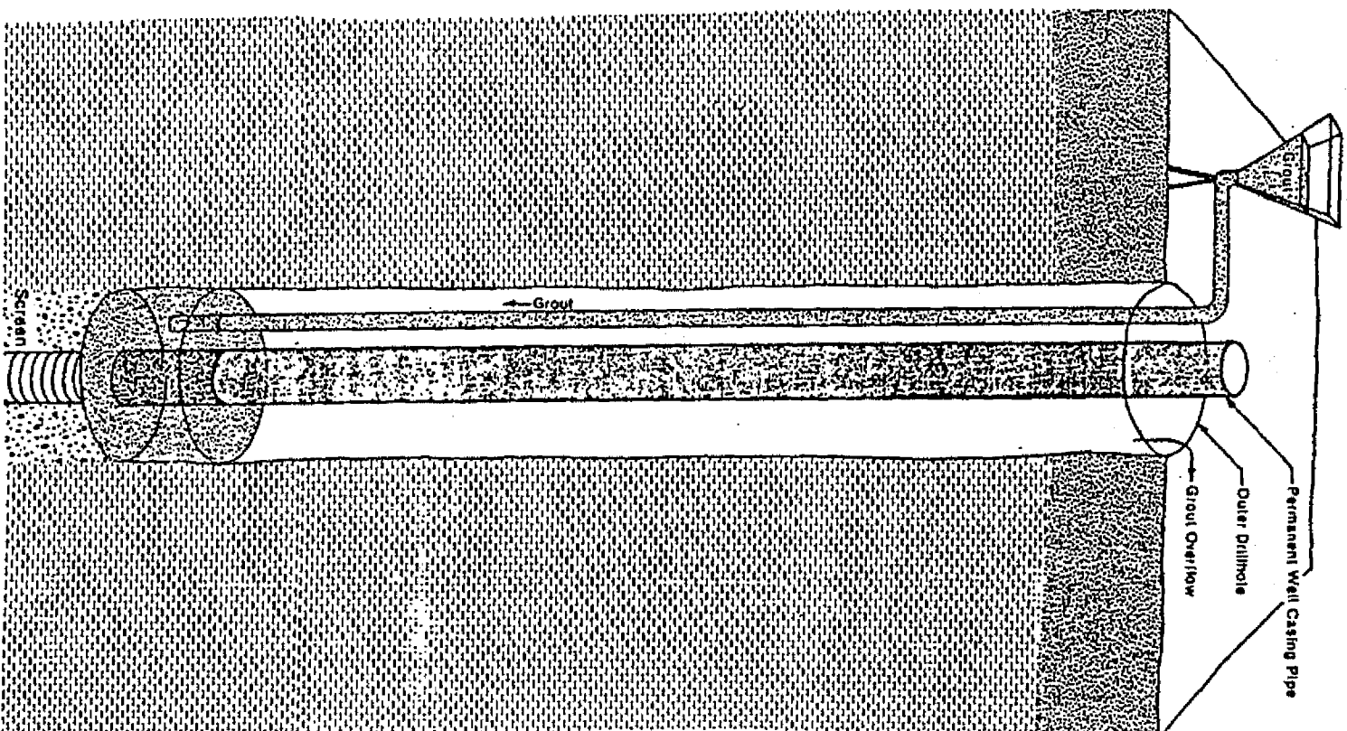
Figure 2. Conductor (tremie) pipe — gravity method
