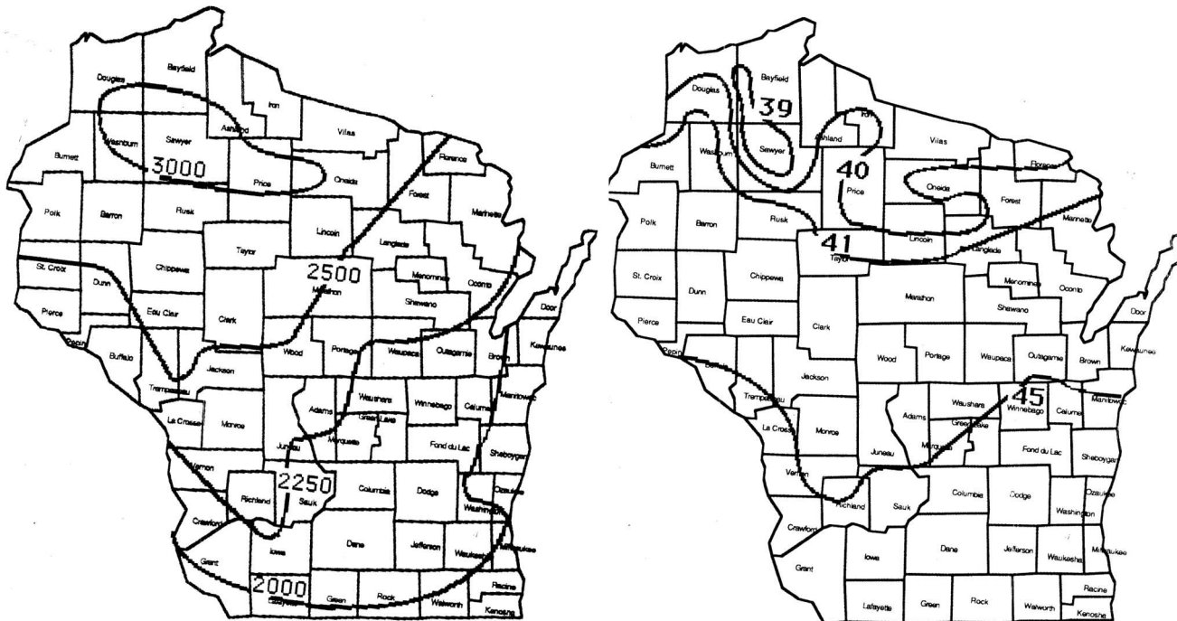
Air-Freeze Index Contour Map
