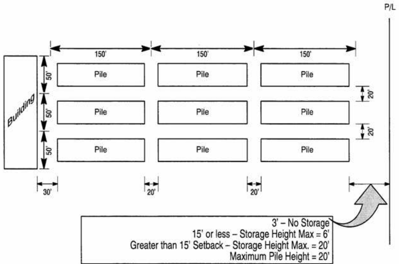
A-314.10 (2) OUTSIDE STORAGE SCHEMATIC.
