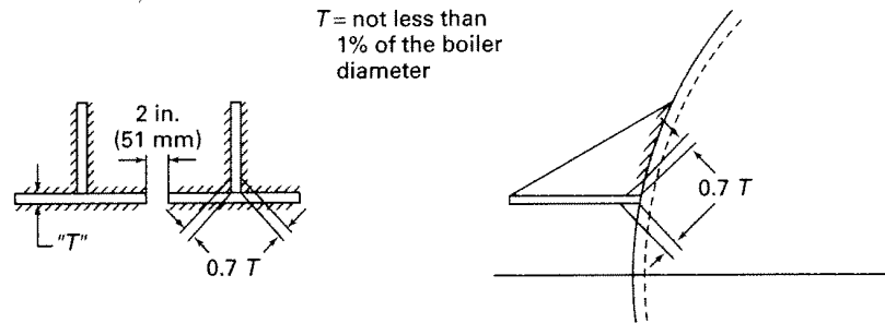
FIG. HG-725(b) WELDED BRACKET CONNECTION FOR HORIZONTAL-RETURN TUBULAR BOILER
