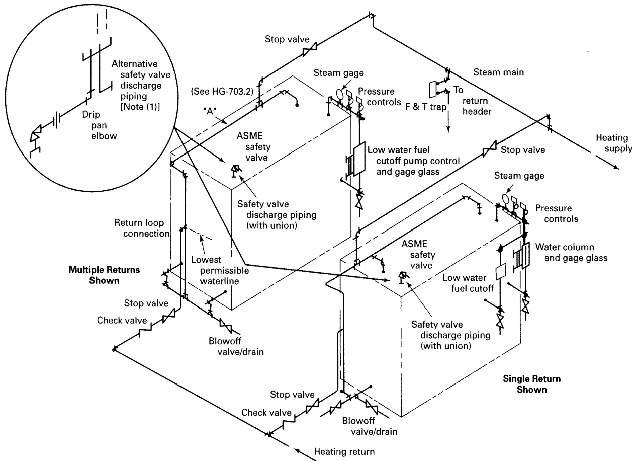
FIG. HG-703.1(b) STEAM BOILERS IN BATTERY – GRAVITY RETURN – ACCEPTABLE PIPING INSTALLATION
