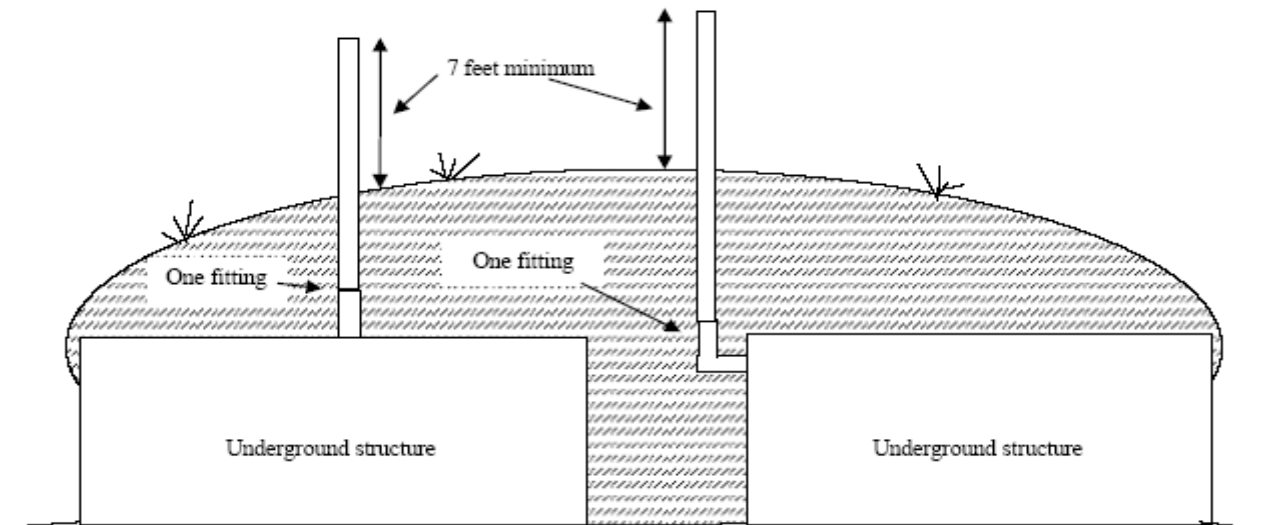
VENTS TERMINATING FOR UNDERGROUND STRUCTURES
