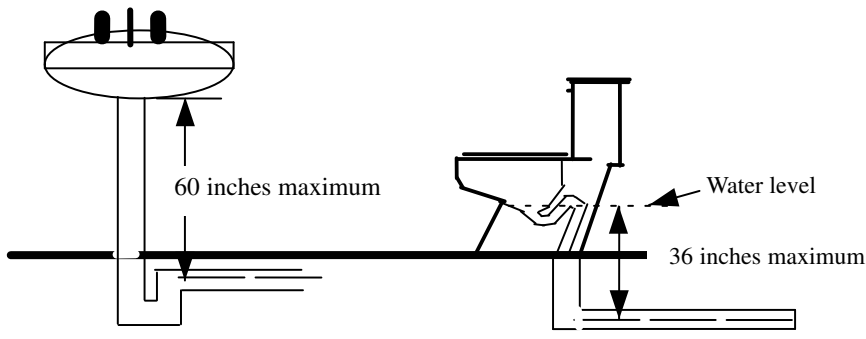
Pedestal fixtures (Lavatory, shampoo sink, drinking fountain or cuspidor)
