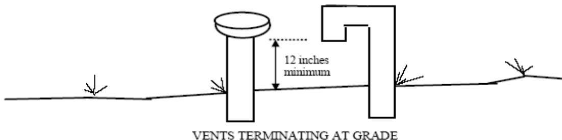
VENTS TERMINATING AT GRADE
