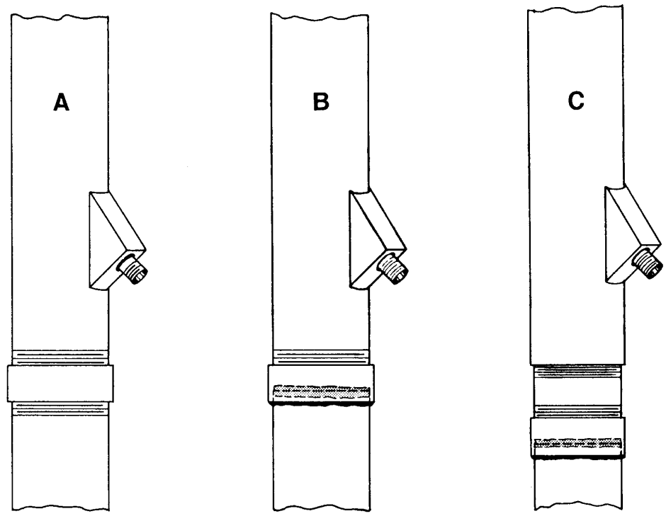
Figure 30. Pitless unit connections for wells with steel well casing pipe.
