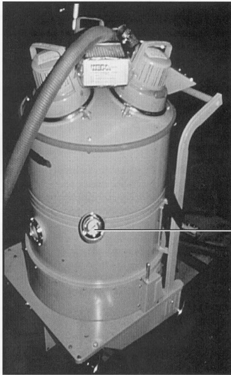
Figure 14.1b Pressure Gauge Indicator Shows When Filters Require Changing.
