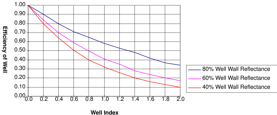
Figure 63.1005 Well Efficiency
