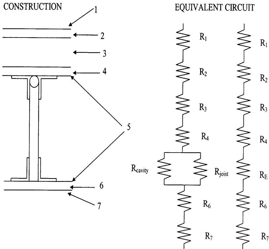
Calculation Procedure for Thermal Resistance of a Typical Roof Assembly
