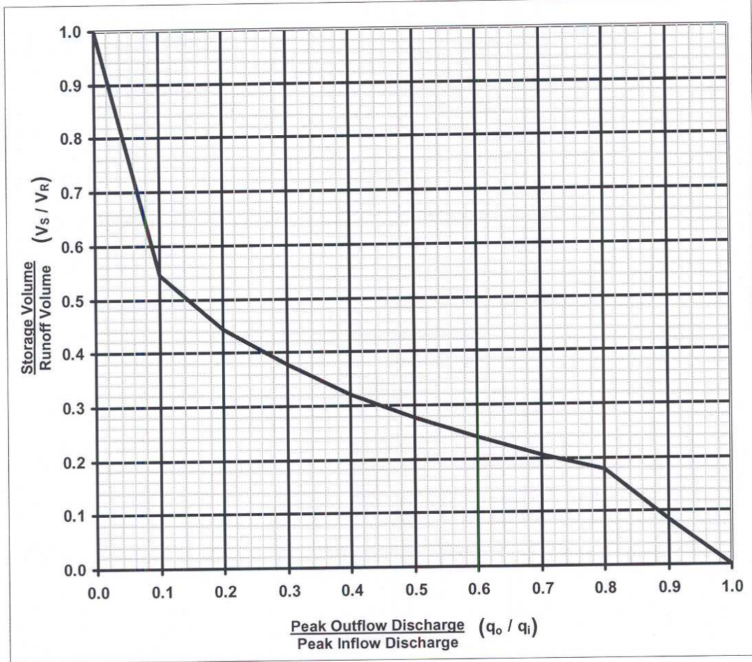
Figure 2 Approximate Detention Basin Routing for Type II Storms
