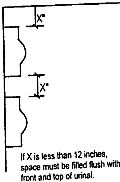
Figure A-84.20-4. Spacing between urinals.
