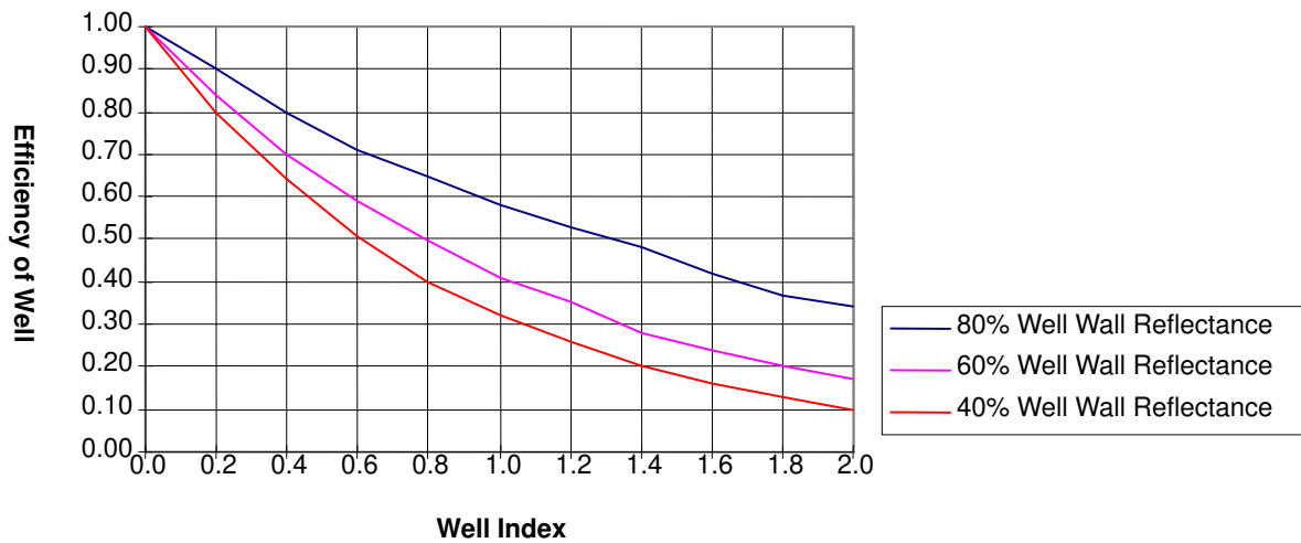
Figure 63.1005 Well Efficiency
