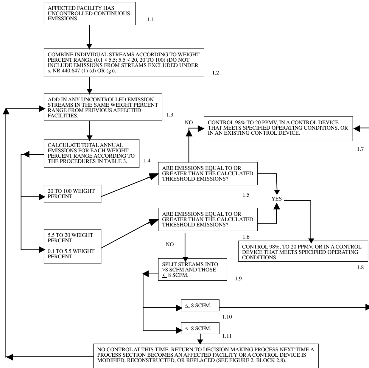
Figure 1. Decision Making Process for Uncontrolled Continuous Emissions from Polypropylene and Polyethylene Affected Facilities
