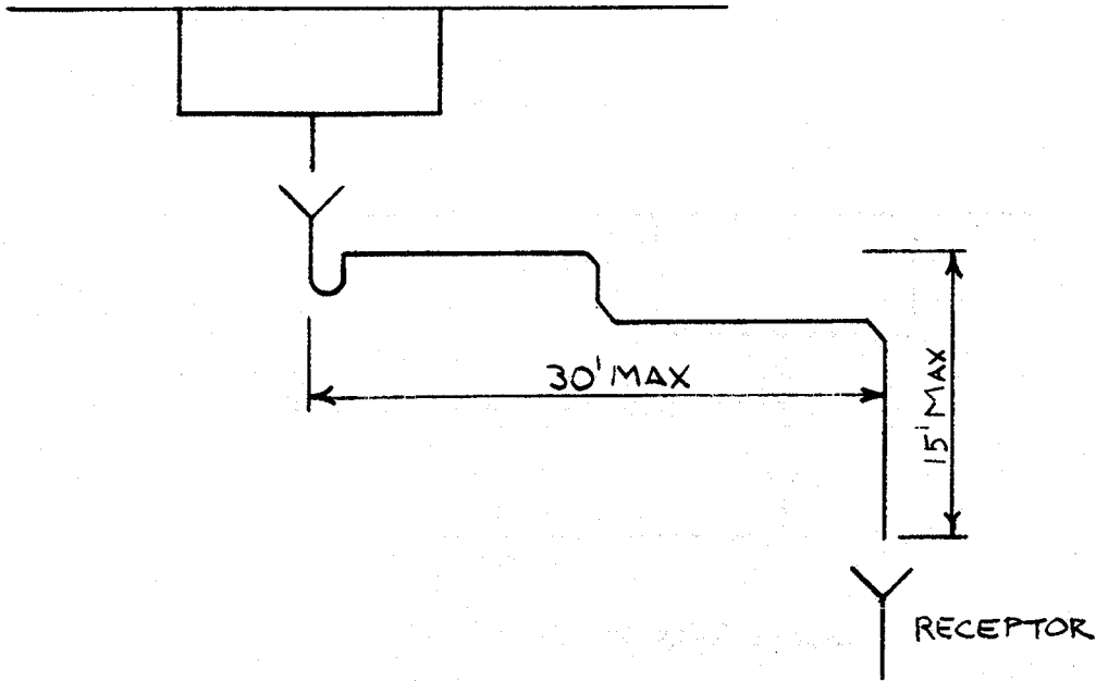
MAXIMUM LENGTH OF LOCAL WASTE PIPE
