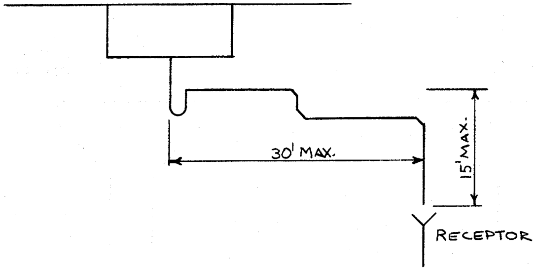
MAXIMUM LENGTH OF INDIRECT WASTE PIPE
