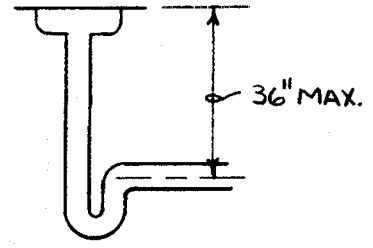
FLOOR DRAIN
