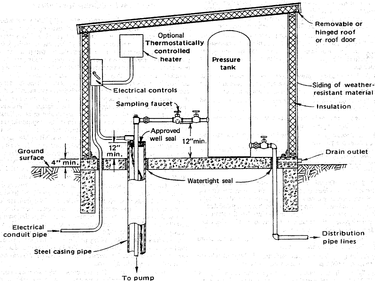
Figure 46. Pumphouse specifications.
