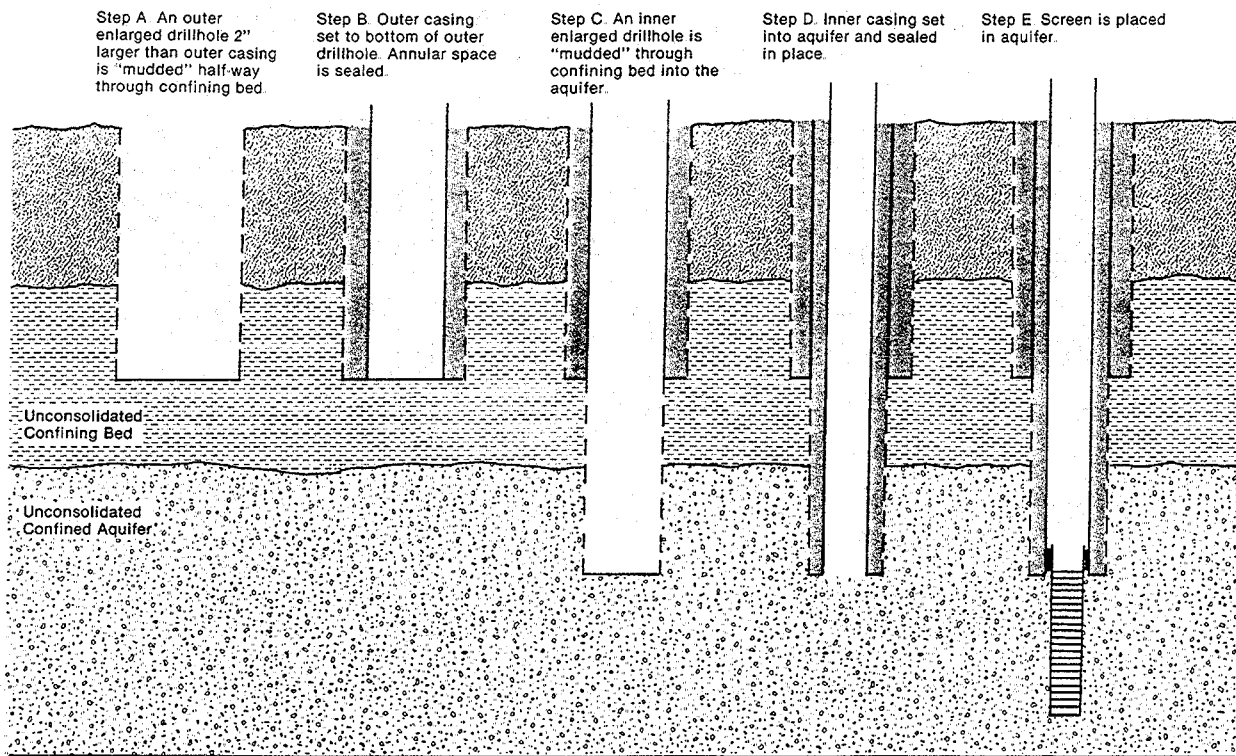
Figure 7. (b) 2. Rotary method for flowing well construction—confined aquifer more than 40@ feet below the ground surface—both confining bed and aquifer are unconsolidated—double casing construction.
