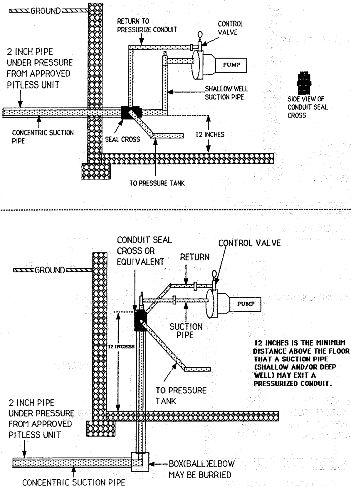
Figure 36c. Alternate offset pump installation discharge piping using a buried box (ball) elbow and seal cross fitting. Figure prepared by I. Roos.
