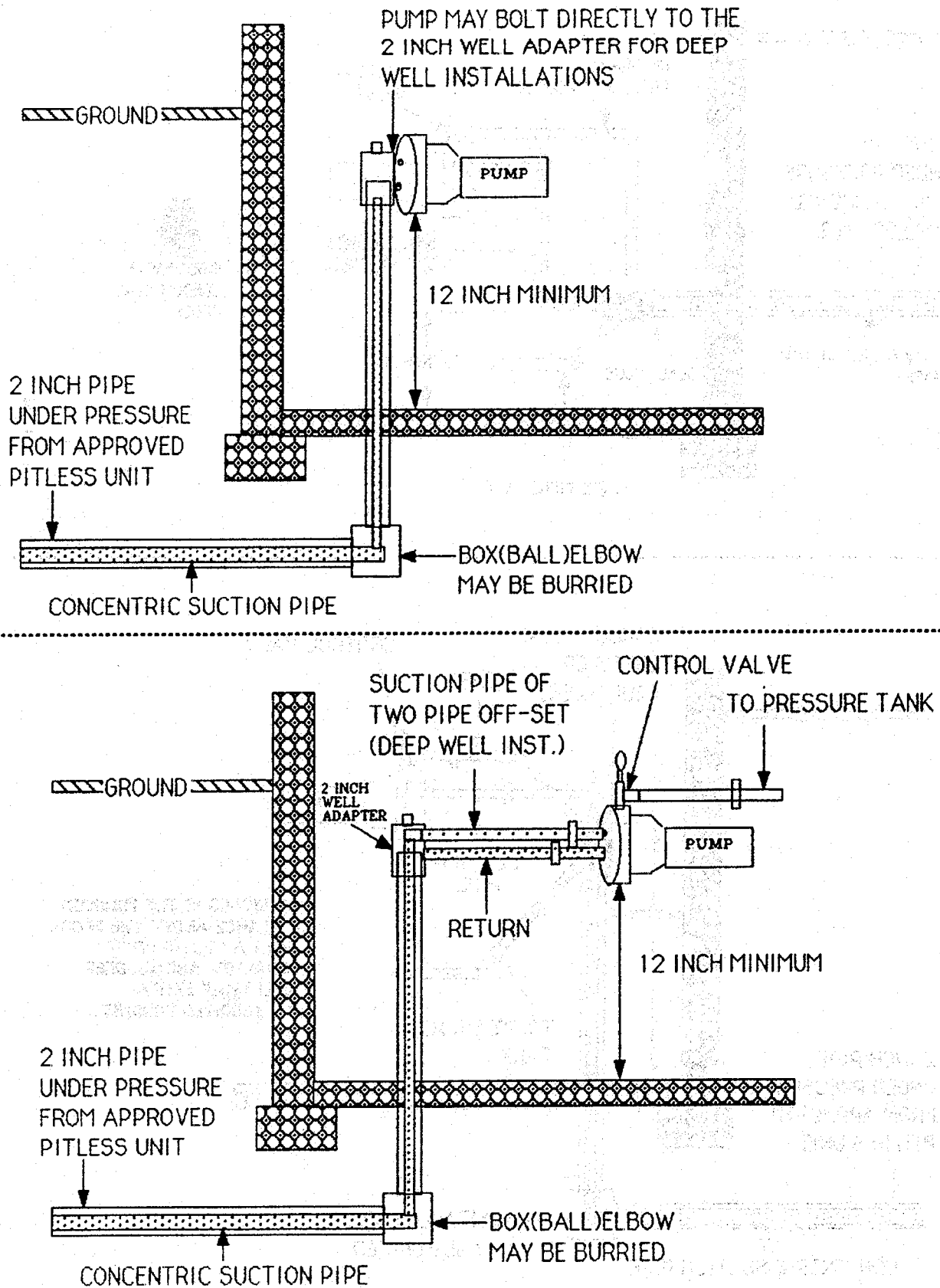
Figure 36b. Offset pump installation discharge piping using a buried box (ball) elbow. Figure prepared by I. Roos.
