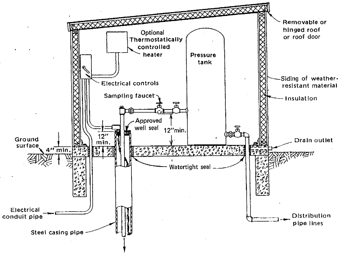
Figure 46. Pumphouse specifications.
