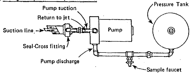
Figure 35. Pump installation for a deep well jet pump assembly with a pressure conduit having a concentric piping arrangement. A pressure (box) elbow may be used to extend the pressurized conduit to a point above the basement floor. The pressure (box) elbow may be buried.
