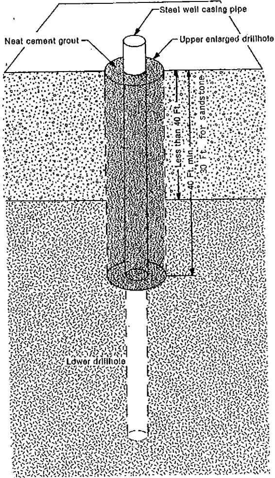
Figure 61. Line E. Rotary methods for low capacity* and nonpotable high capacity wells in all types of bedrock with less than 40 feet of overlying casing material.
