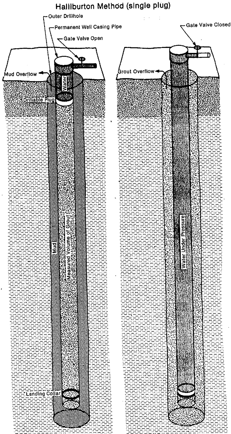
Figure 16. Halliburton (single plug) method for neat cement grouting.
