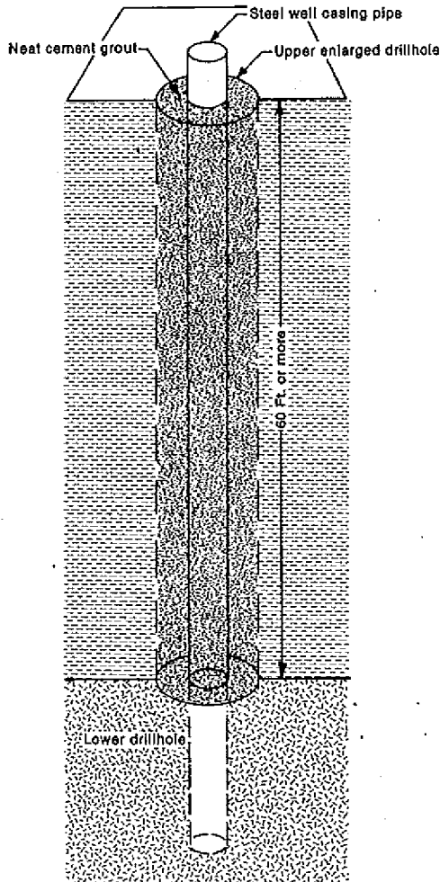
Figure 71. Line J. Rotary methods for potable high capacity, school, and wastewater treatment plant wells in all types of bedrock with at least 60 feet of overlying non-caving material. The diameter of the upper enlarged drillhole shall be at least 3 inches larger than the outside diameter of the well casing pipe or well casing pipe couplings, if used. The diameter of the well casing pipe and lower drillhole shall be at least 6 inches. During construction the upper enlarged drillhole shall be maintained at full diameter by circulating drilling mud.
