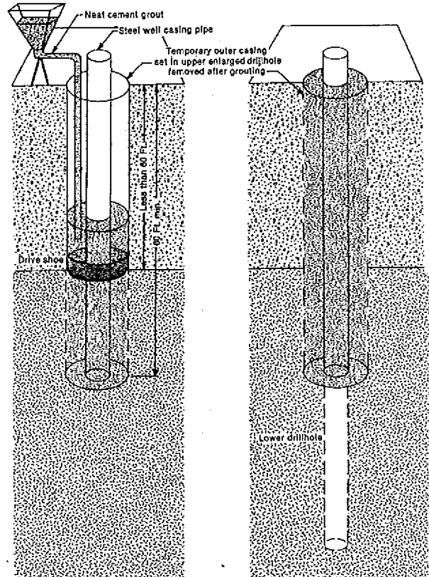
Figure 72. Line K. Percussion methods for potable high capacity, school, and wastewater treatment plant wells in all types of bedrock with less than 60 feet of overlying caving material. The diameter of the upper enlarged drillhole shall be at least 3 inches larger than the outside diameter of the well casing pipe or well casing pipe couplings, if used. The diameter of the well casing pipe and lower drillhole shall be at least 6 inches.
