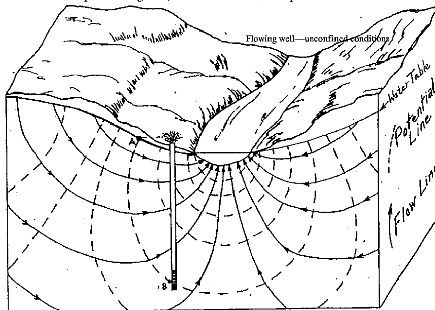
Figure 3. A flowing well in an unconfined aquifer.
