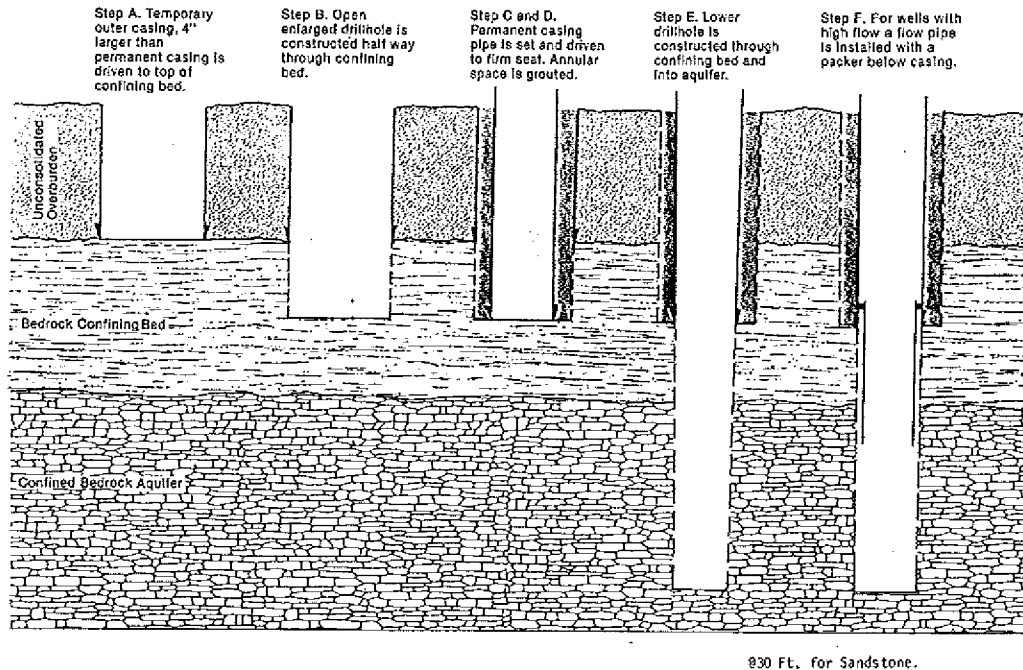
Figure 9. (c) 1. Percussion method for flowing well construction—confined bedrock aquifer more than 40 feet below the ground surface with a bedrock confining bed.
