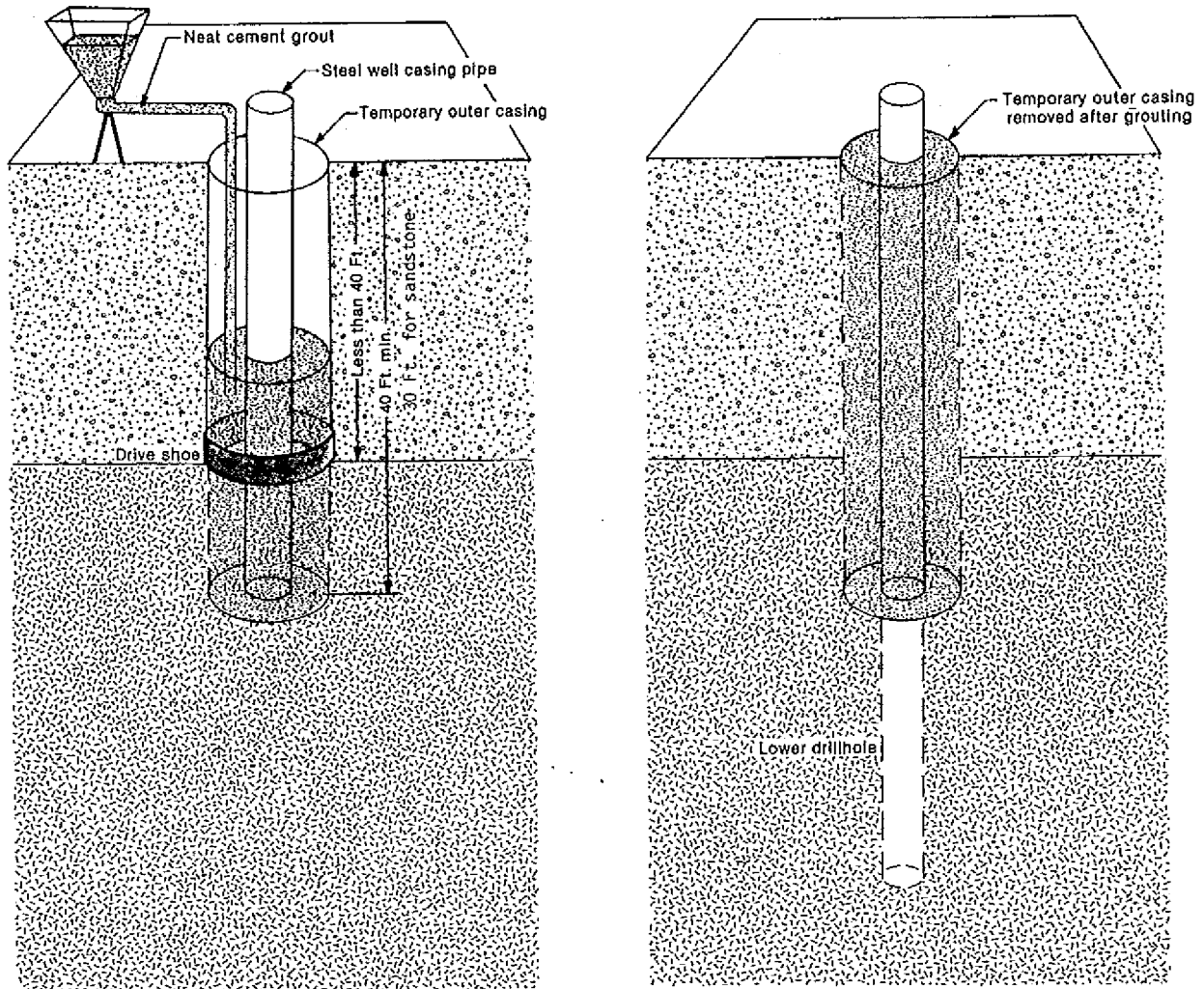
Figure 60. Line E. Percussion methods for low capacity* and nonpotable high capacity wells in all types of bedrock with less than 40 feet of overlying caving material. *Not including school or wastewater treatment plant wells. For well casing pipe with welded joints only. For threaded and coupled well casing pipe the diameter shall be at least 4 inches larger than the nominal diameter of the well casing pipe.
