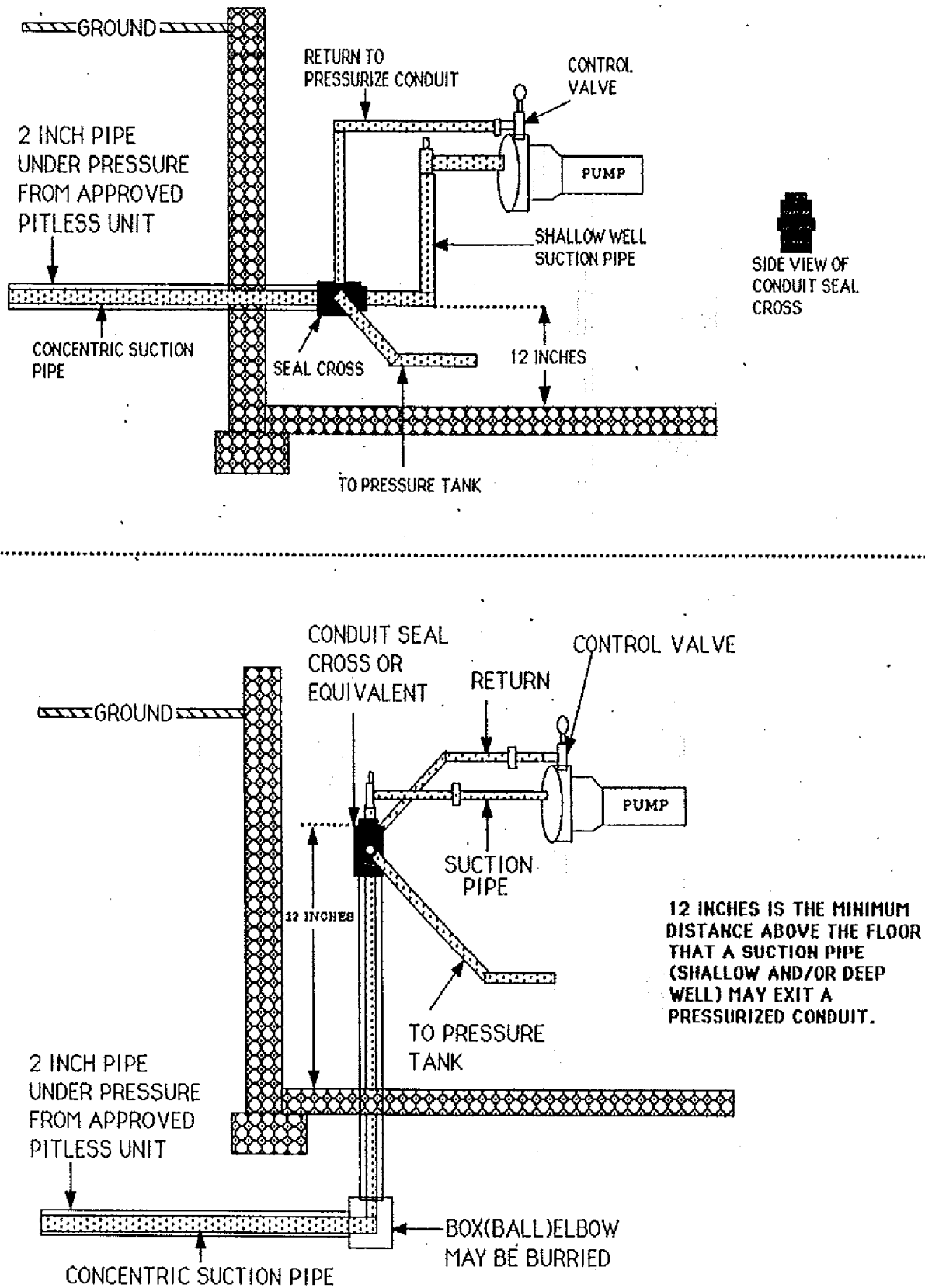
Figure 36c. Alternate offset pump installation discharge piping using a buried box (ball) elbow and seal cross fitting. Figure prepared by T. Roos.
