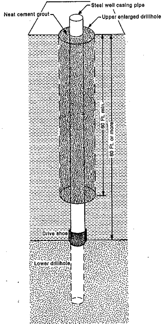
Figure 70. Line I. Percussion methods for potable high capacity, school, and wastewater treatment plant wells in all types of bedrock with at least 60 feet of overlying non-caving material.
