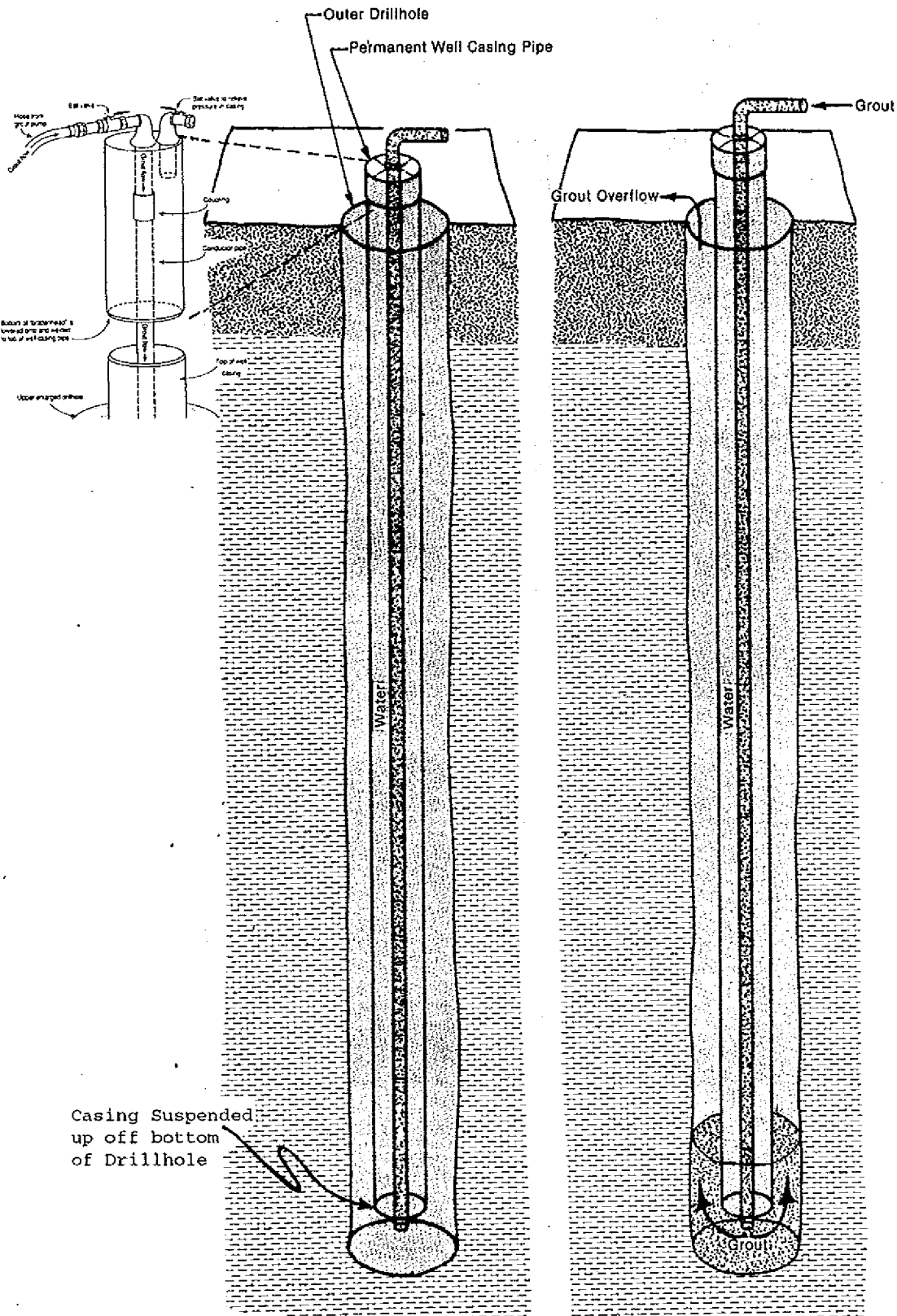
Figure 14. Well seal/conductor (tremie) pipe-pumped (Braden-Head) method for neat cement grouting.
