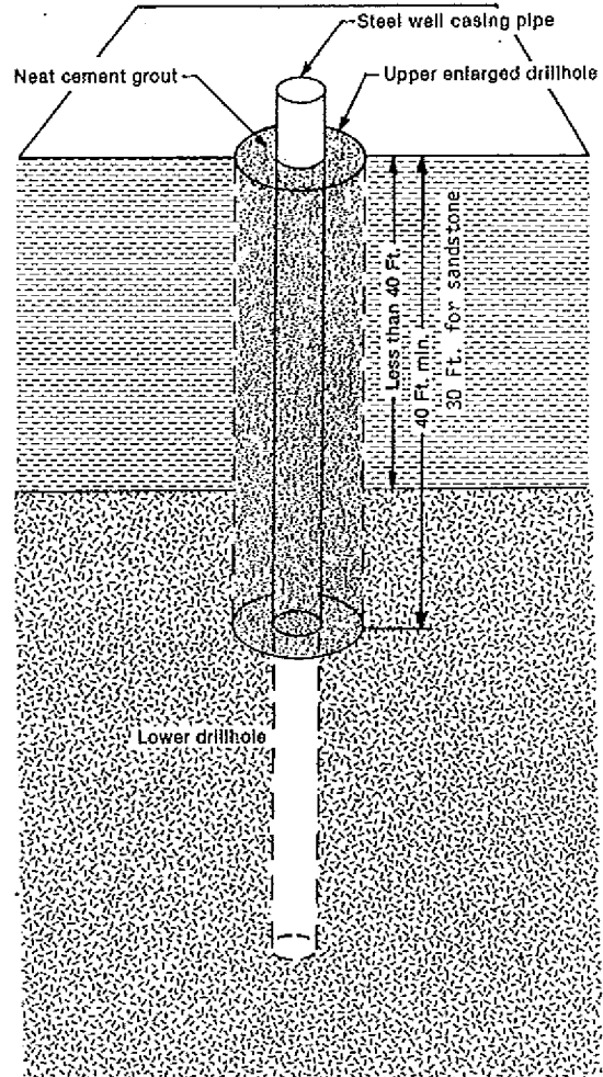
Figure 62. Line B. Rotary methods for low capacity* and nonpotable high capacity wells in all types of bedrock with less than 40 feet of overlying non-caving material. *Not including school or wastewater treatment plant wells.
