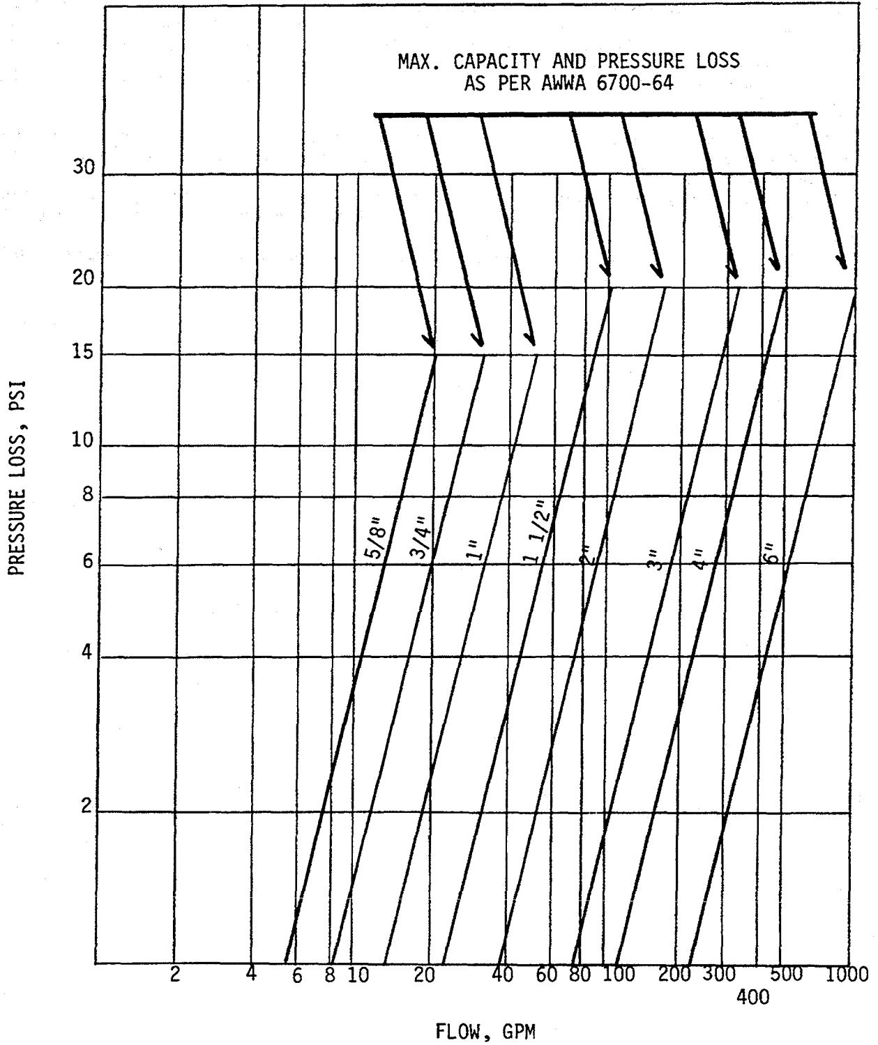
Graph A-82.40 (7) - 1 PRESSURE LOSS IN COLD-WATER METERS, DISPLACEMENT TYPE
