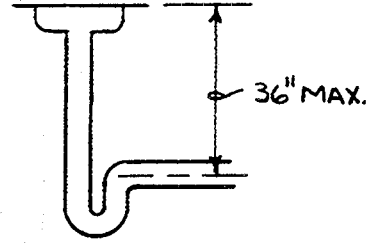
FLOOR DRAIN
