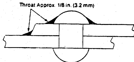
Figure 42.10-2 SEAL WELDING OF RIVETED JOINTS
