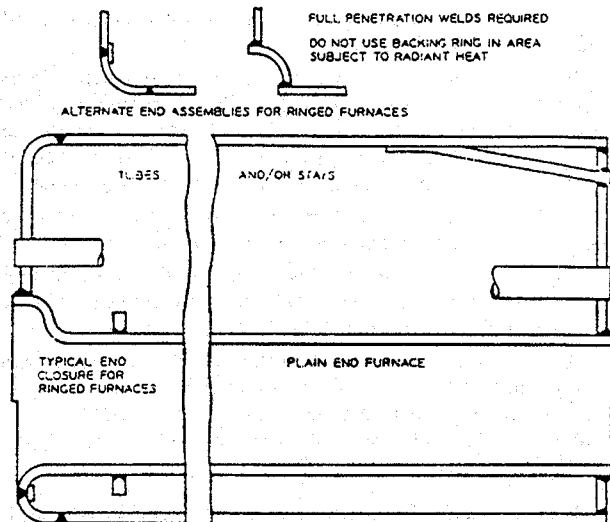
Figure 42.19-2 ACCEPTABLE FURNACE RENEWAL
