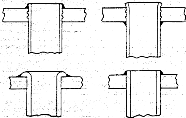
Figure 42.10-1 SEAL WELDING OF TUBES
