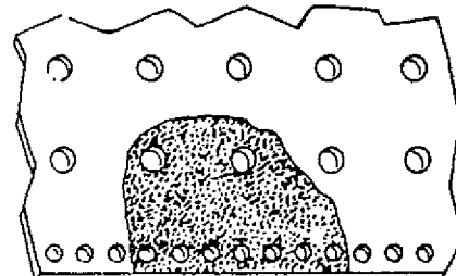
Figure 42.09-1 WELD BUILD-UP OF WASTED AREAS
