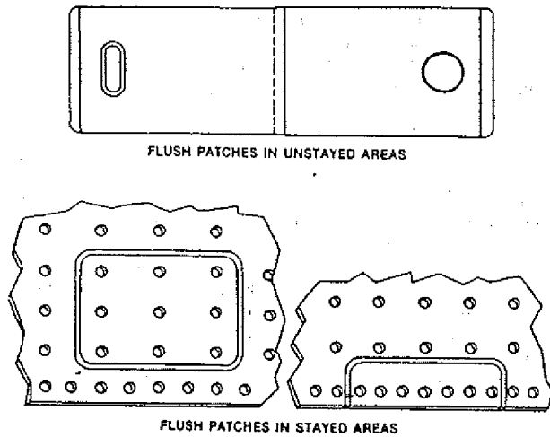
Figure 42.17-1 FLUSH PATCHES
