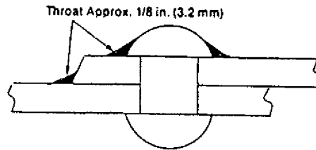
Figure 42.10-2 SEAL WELDING OF RIVETED JOINTS
