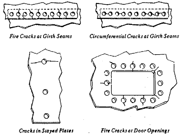
Figure 42.08-1 RIVET AND STAYBOLT HOLE CRACKS
