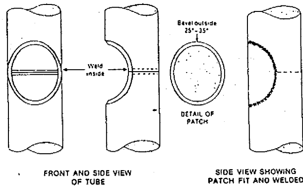
Figure 42.17-2 TUBE WINDOW PATCHING METHOD
