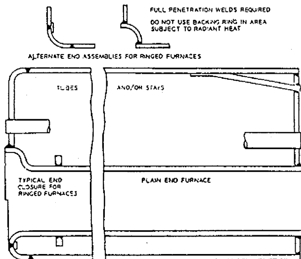
Longitudinal seam in furnace double butt-welded and thermally stress-relieved
