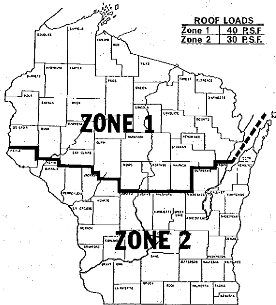
Zone Map for Roof Loads
