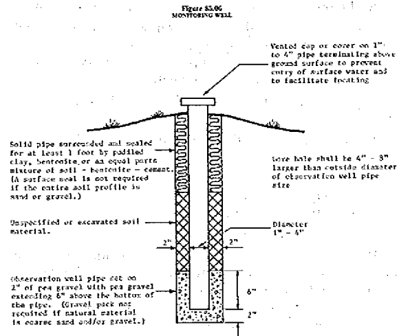
Figure 85.06 MONITORING WELL
