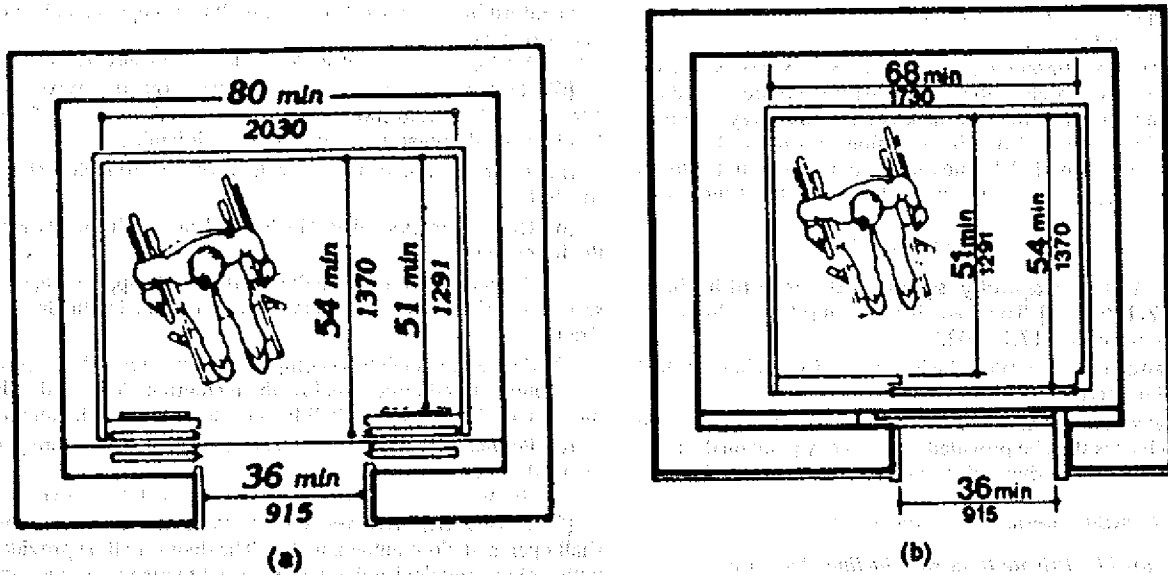
FIGURE 18.83-A Minimum Dimensions of Elevator Cars
