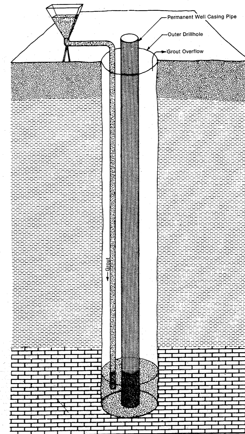
Figure 11. Conductor (tremie) pipe-gravity method for neat cement grouting.
