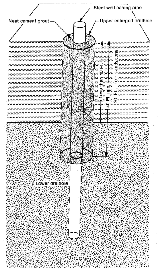
Figure 62. Line E. Rotary methods for low capacity* and nonpotable high capacity wells in all types of bedrock with less than 40 feet of overlying non-caving material.
