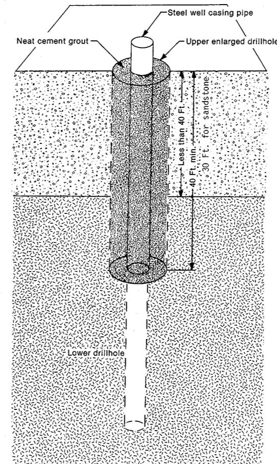
Figure 61. Line E. Rotary methods for low capacity* and nonpotable high capacity wells in all types of bedrock with less than 40 feet of overlying non-caving material.
