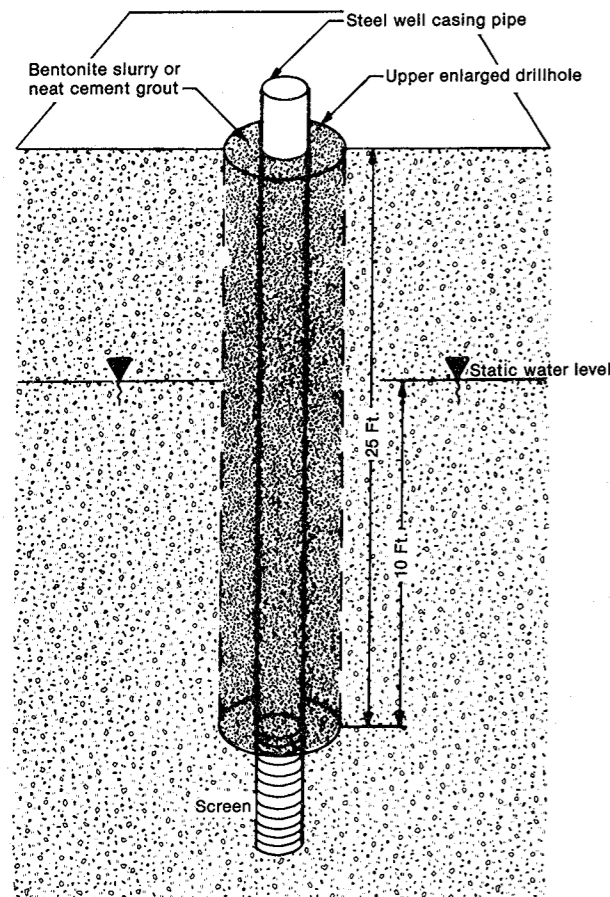
Figure 52. Line A Rotary methods for low capacity* and nonpotable high capacity wells in unconsolidated aquifers overlain by caving material. Well casing pipe shall extend to the 25-foot depth or 10 feet below the static water level, whichever is greater.
