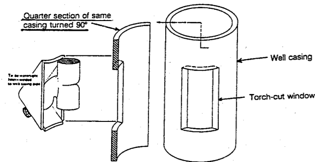
Figure 28. A weld-on pitless adapter.
