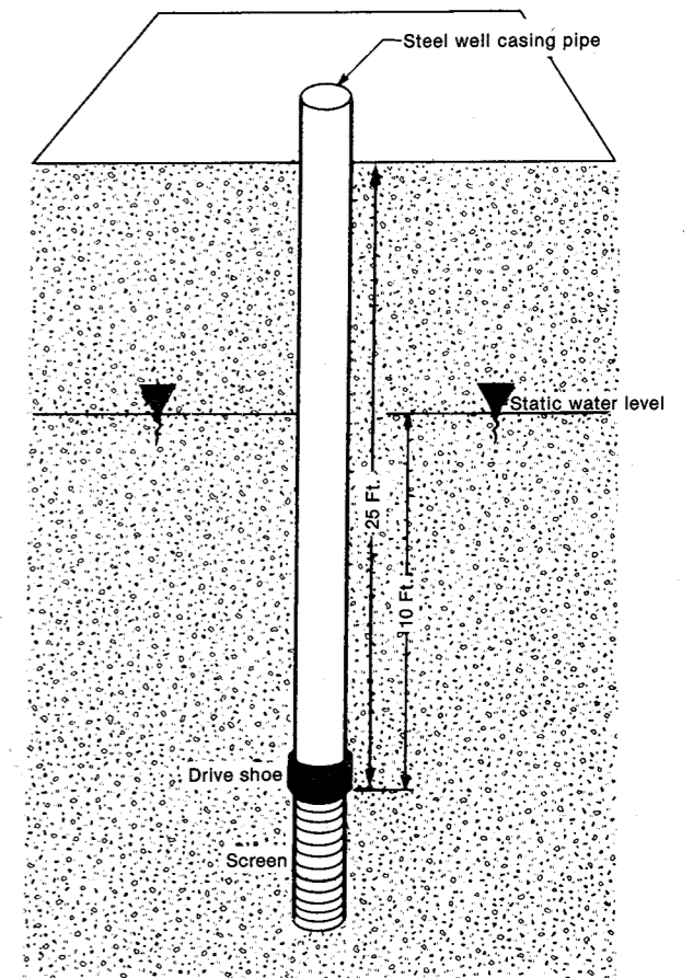
Figure 51 Line A. Percussion methods for low capacity* and nonpotable high capacity wells in unconsolidated aquifers overlain by caving material. Well casing pipe shall extend to the 25-foot depth or 10 feet below the static water level, whichever is greater. The well casing pipe shall be 2 inches minimum diameter and may be driven from the ground surface.
