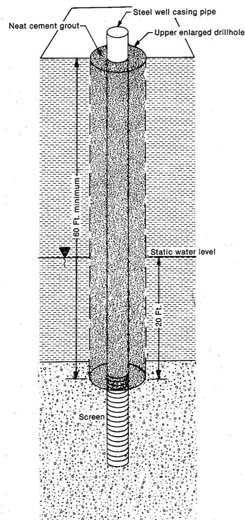
Figure 67. Line H Rotary methods for potable high capacity, school, and wastewater treatment plant wells in unconsolidated aquifers overlain by non-caving material. The well casing shall extend to the 60-foot depth or 20 feet below the static water level, whichever is greater.
