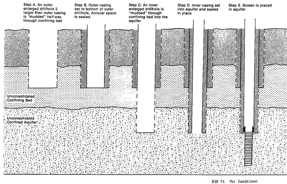
Figure 7. (b) 2. Rotary method for flowing well construction - confined aquifer more than 40 feet below the ground surface - both confining bed and aquifer are unconsolidated - double casing construction.
