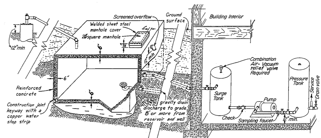
Figure 44A. Reservoir specifications.
