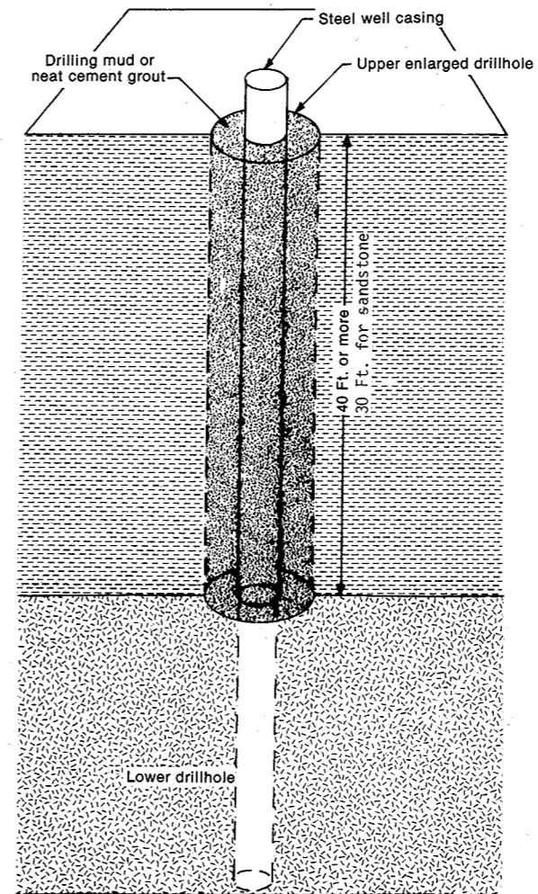
Figure 58. Line D. Rotary methods for low capacity* and nonpotable high capacity wells in all types of bedrock with at least 40 feet of overlying non-caving material.
