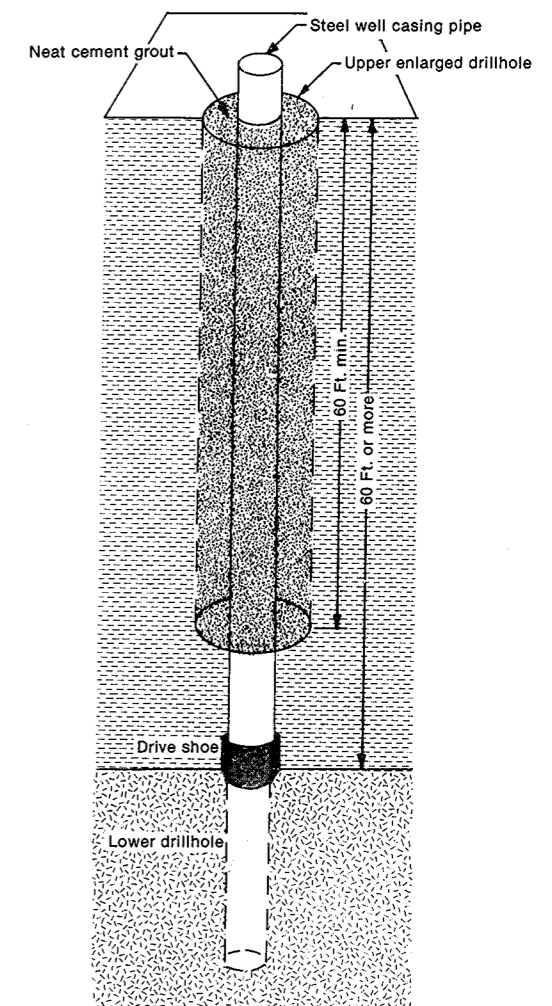
Figure 70. Line J. Percussion methods for potable high capacity, school, and wastewater treatment plant wells in all types of bedrock with at least 60 feet of overlying non-caving material.
