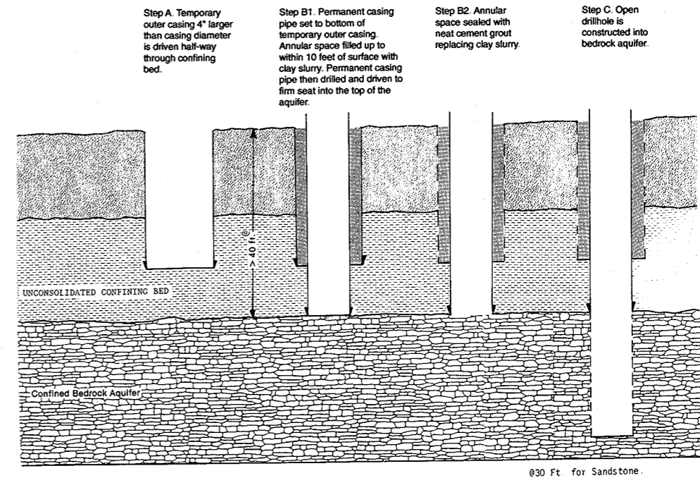
Figure 6. (b) 1. Percussion method for flowing well construction - confined bedrock aquifer more than 40 feet below the ground surface with an unconsolidated confining bed.
