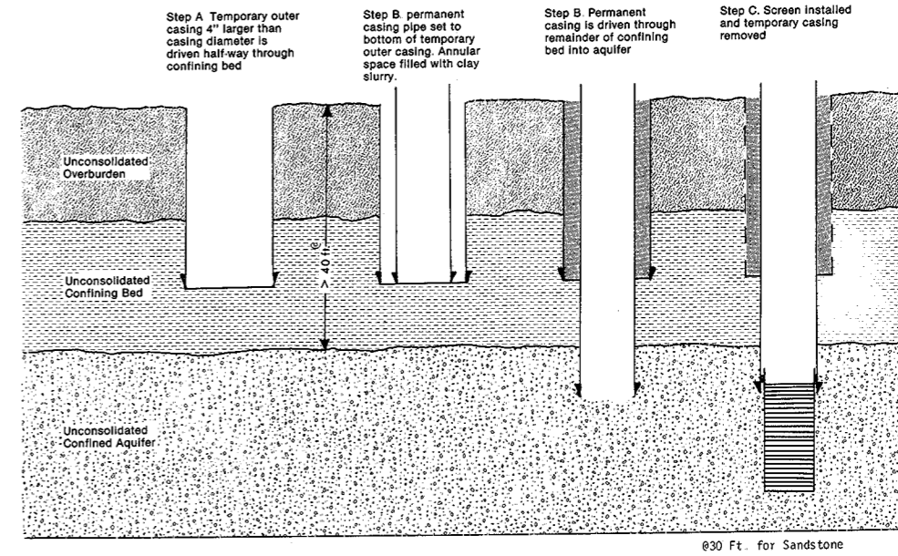
Figure 5. (b) 1. Percussion method for flowing well construction - confined unconsolidated aquifer more than 40 feet below the ground surface with an unconsolidated confining bed.
