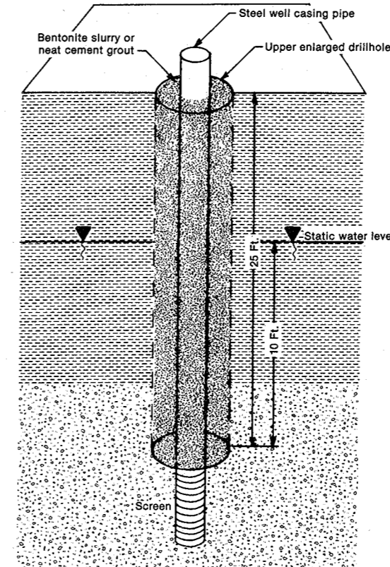
Figure 54. Line B. Rotary methods for low capacity* and nonpotable high capacity wells in unconsolidated aquifers overlain by non-caving material. Well casing pipe shall extend to the 25-foot depth or 10 feet below the static water level, whichever is greater.
