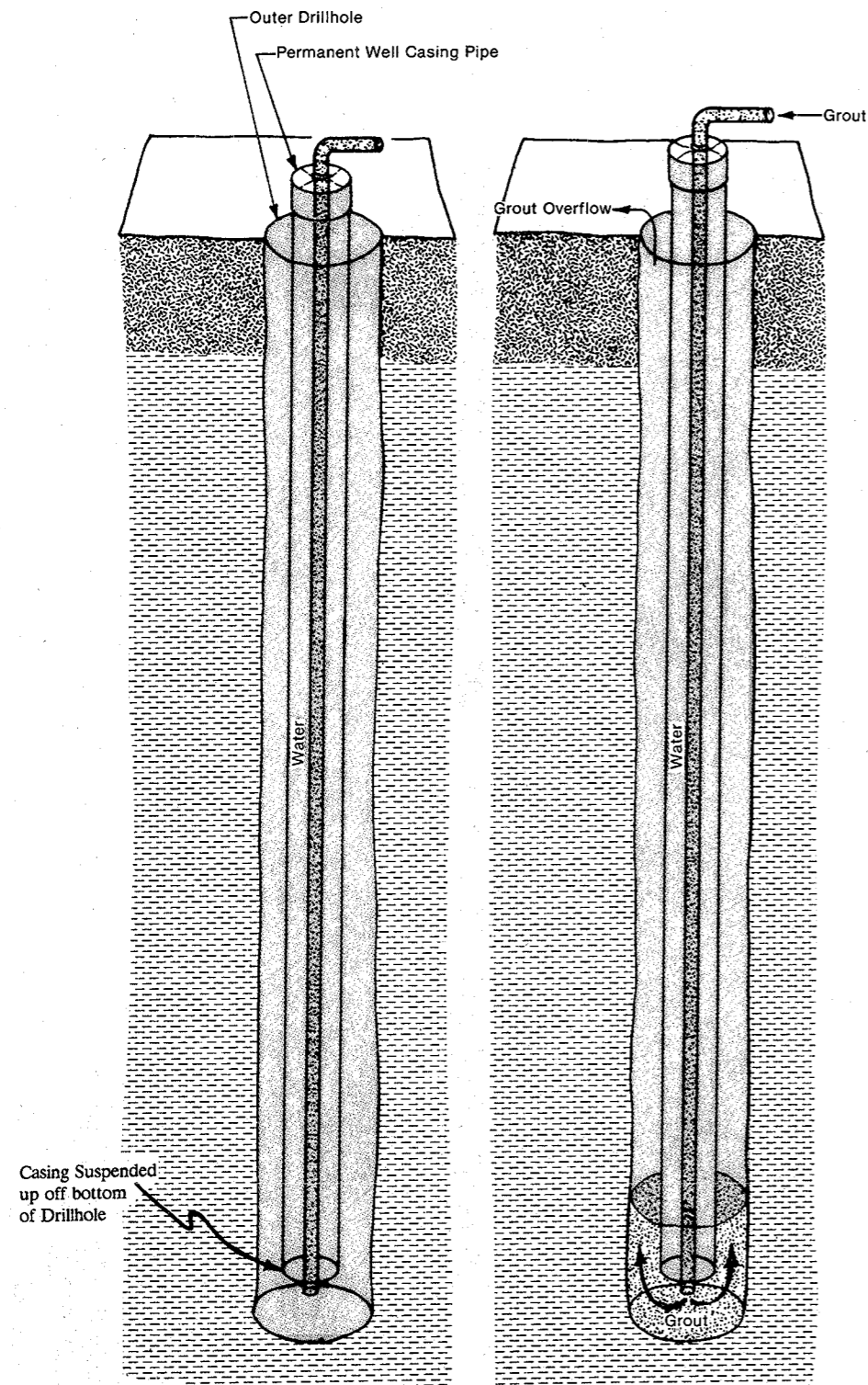
Figure 14. Well seal/conductor (tremie) pipe-pumped (Braden-Head) method for neat cement grouting.
