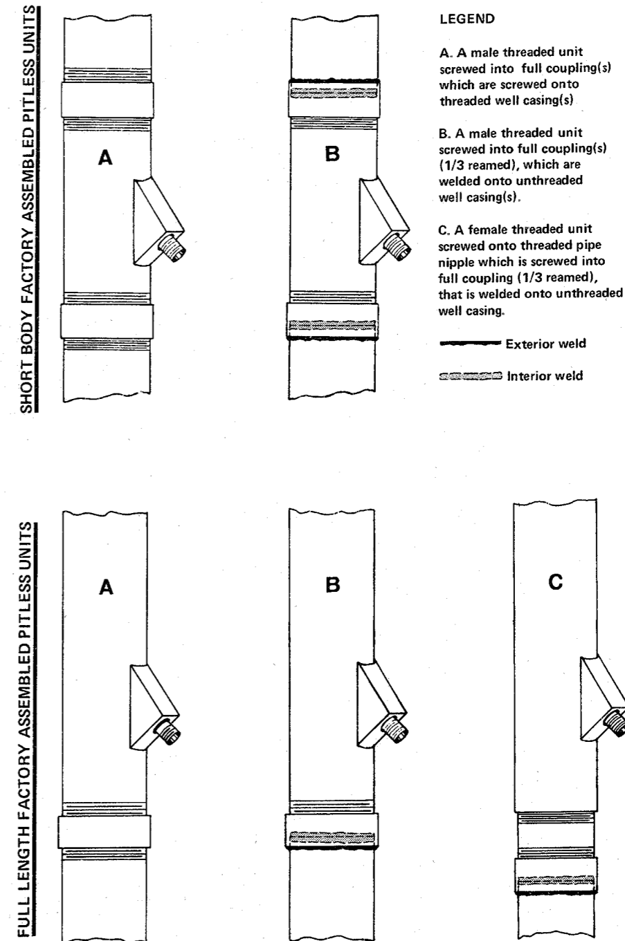
Figure 30. Pitless unit connections for wells with steel well casing pipe. NOTE: A well casing pipe nipple, 1/2 threaded-1/2 beveled may be used in lieu of a full pipe coupling.
