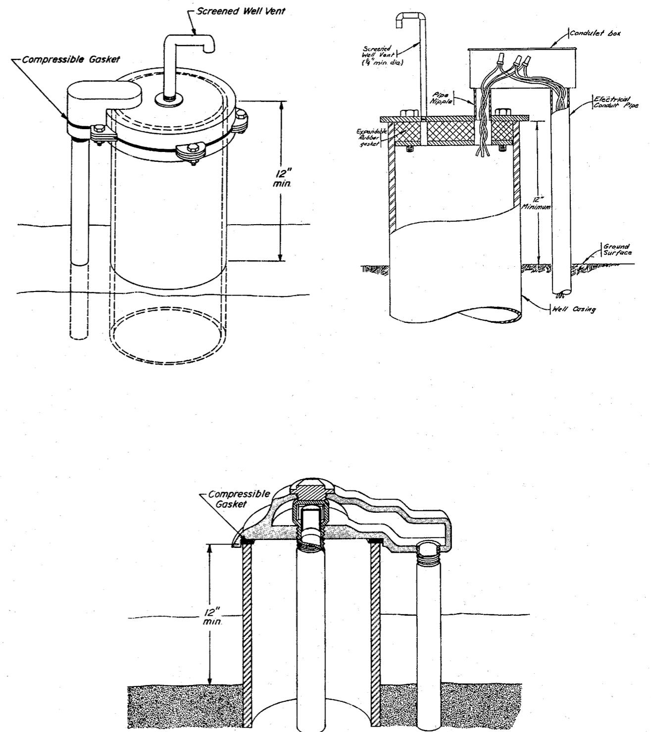
Figure 23. Examples of sanitary well seals.
