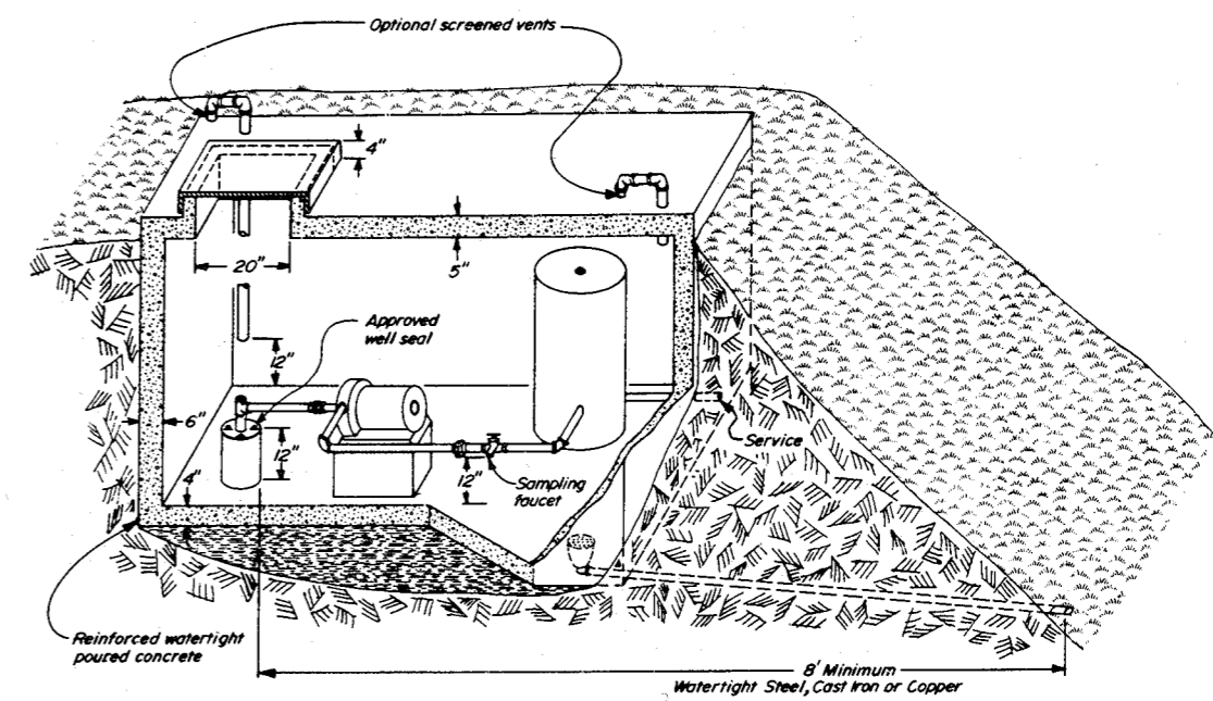
Figure 45. Minimum requirements for approved new well pits.
