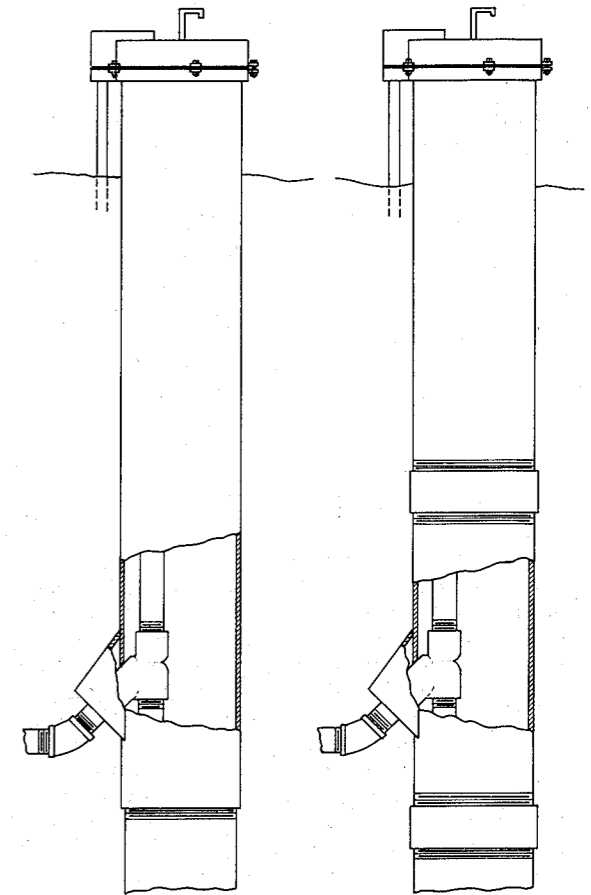
Figure 27. Non-spool type pitless units. (For acceptable procedures for connection of the units to the well casing pipe see s. NR 812.31 (3)).
