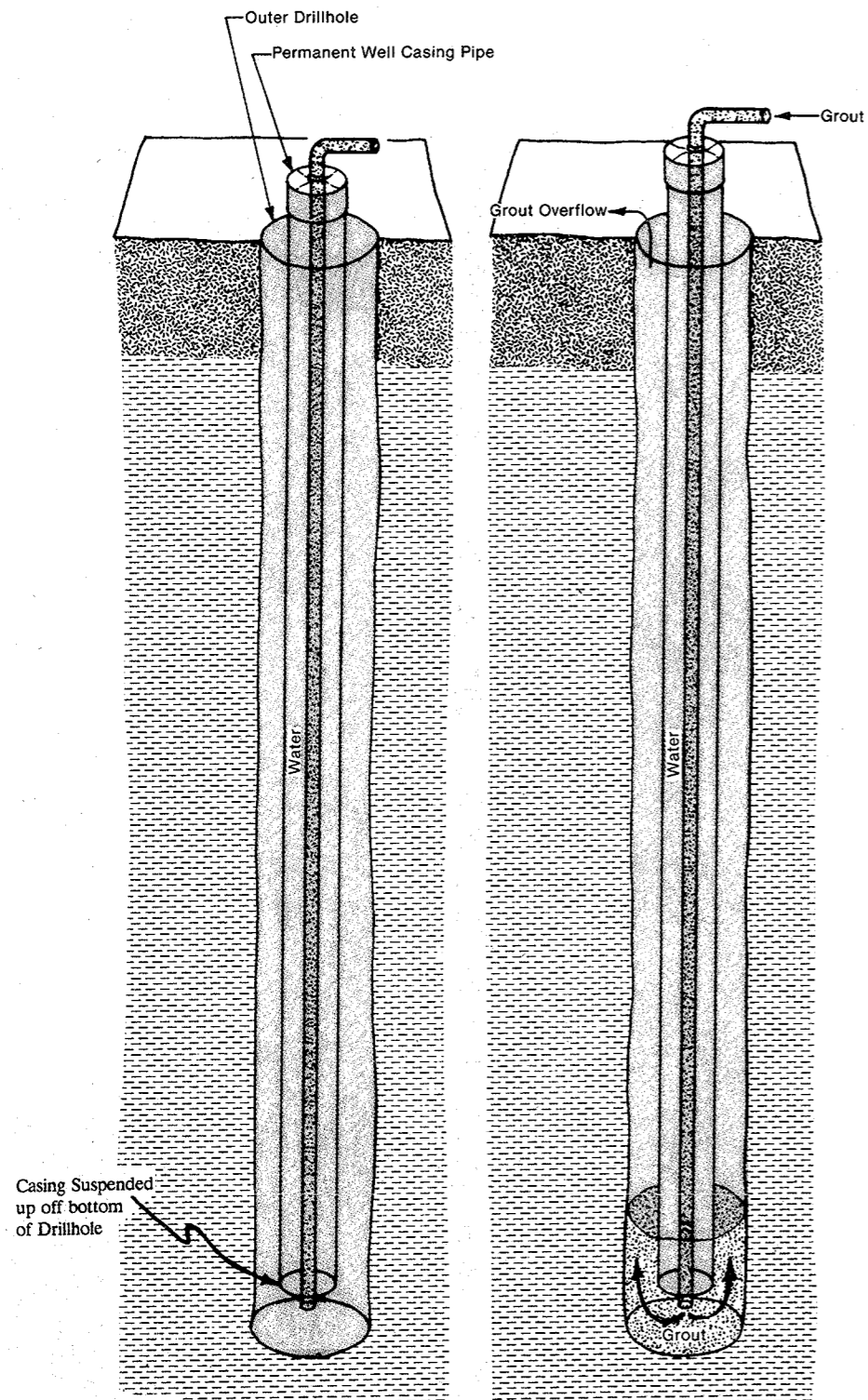
Figure 14. Well seal/conductor (tremie) pipe-pumped (Braden-Head) method for neat cement grouting.
