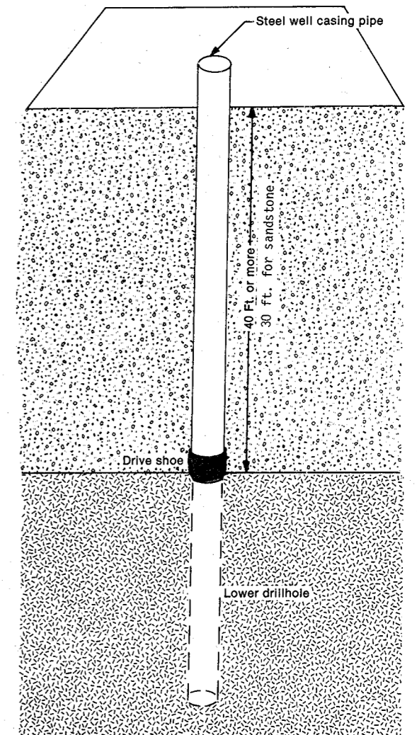
Figure 55. Line C. Percussion methods for low capacity* and nonpotable high capacity wells in all types of bedrock with at least 40 feet of overlying caving material.
