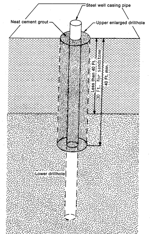
Figure 59. Line E. Percussion methods for low capacity* and nonpotable high capacity wells in all types of bedrock with less than 40 feet of overlying non-caving material.
