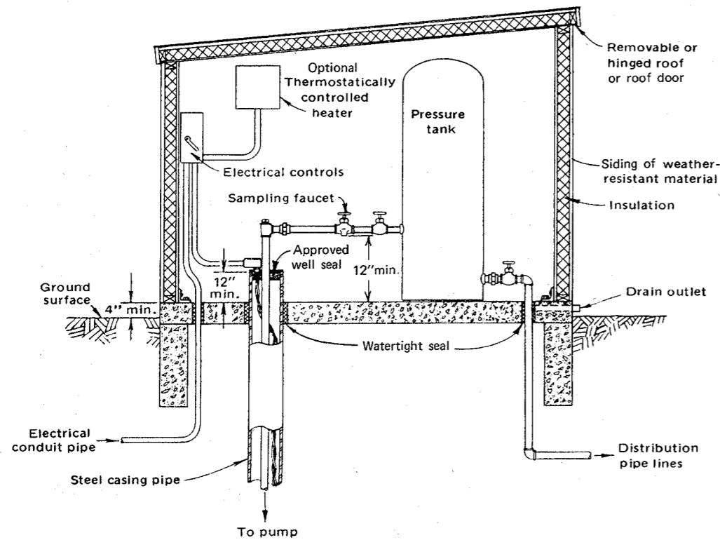
Figure 46. Pumphouse specifications.
