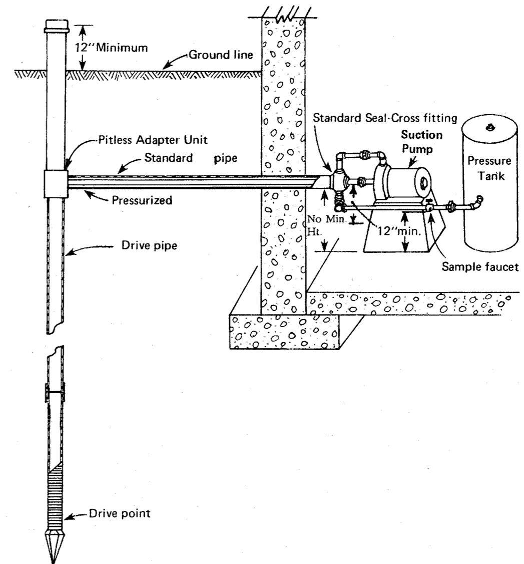
Figure 34. Shallow-well pump installation for a driven-point well. A pressure (box) elbow may be used to extend the pressurized conduit to a point above the basement floor. The pressure (box) elbow may be buried.
