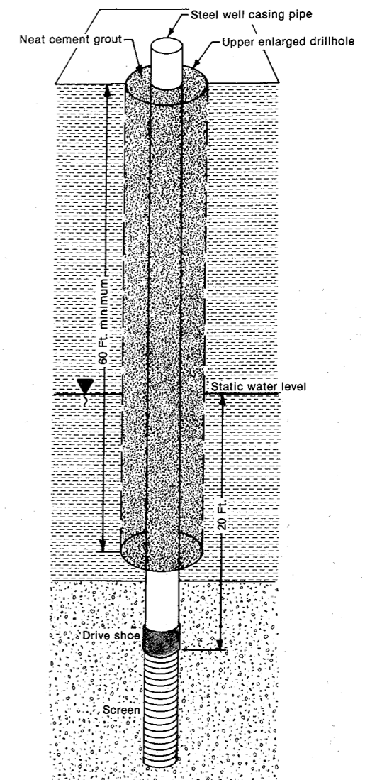
Figure 66. Line H Percussion methods for potable high capacity, school, and wastewater treatment plant wells in unconsolidated aquifers overlain by non-caving material. The well casing pipe shall extend to the 60-foot depth or 20 feet below the static water level, whichever is greater.
