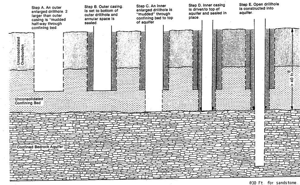
Figure 8 (b) 2. Rotary method for flowing well construction - confined bedrock aquifer more than 40 ft below the ground surface with an unconsolidated confining bed.
