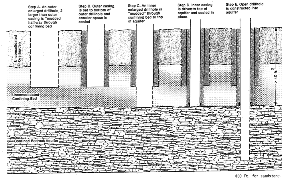
Figure 8. (b) 2 Rotary method for flowing well construction - confined bedrock aquifer more than 40 0 feet below the ground surface with an unconsolidated confining bed.
