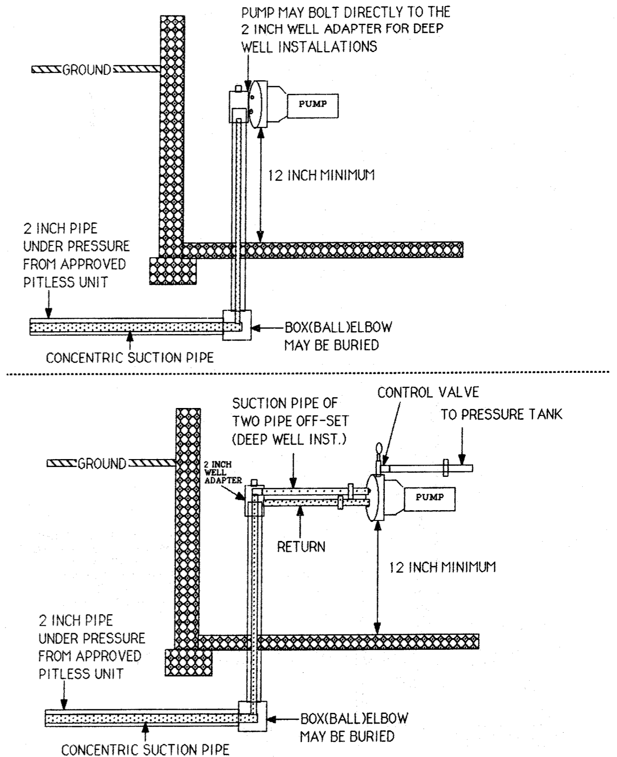
Figure 36b. Offset pump installation discharge piping using a buried box (ball) elbow. Figure prepared by T. Roos.
