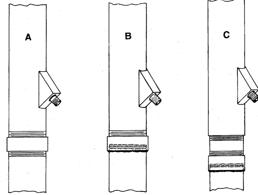
Figure 30. Pitless unit connections for wells with steel well casing pipe. NOTE: A well casing pipe nipple, 1/2 threaded-1/4 beveled may be used in lieu of a full pipe coupling.
