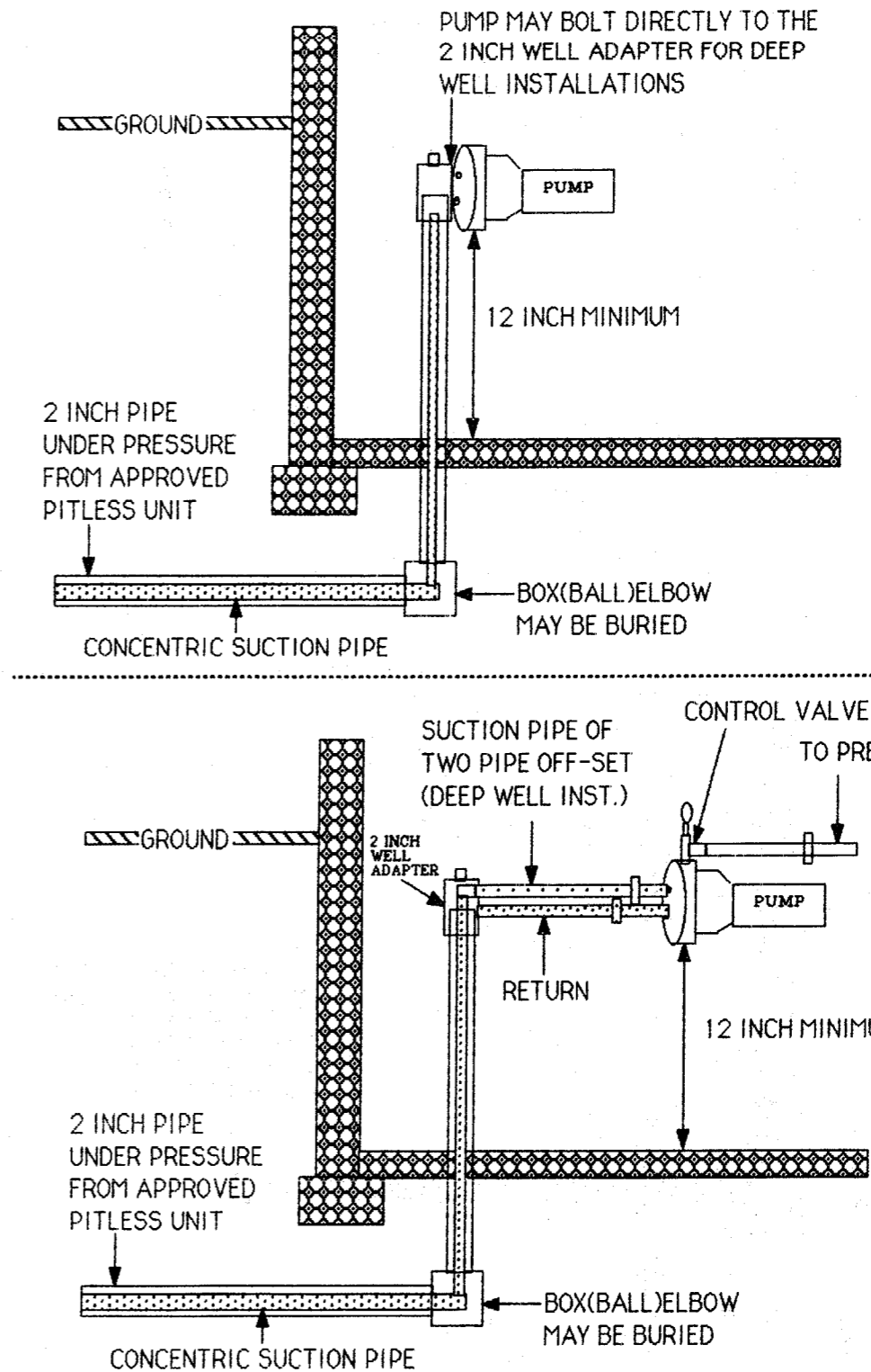
Figure 36b. Offset pump installation discharge piping using a buried box (ball) elbow. Figure prepared by T. Roos.
