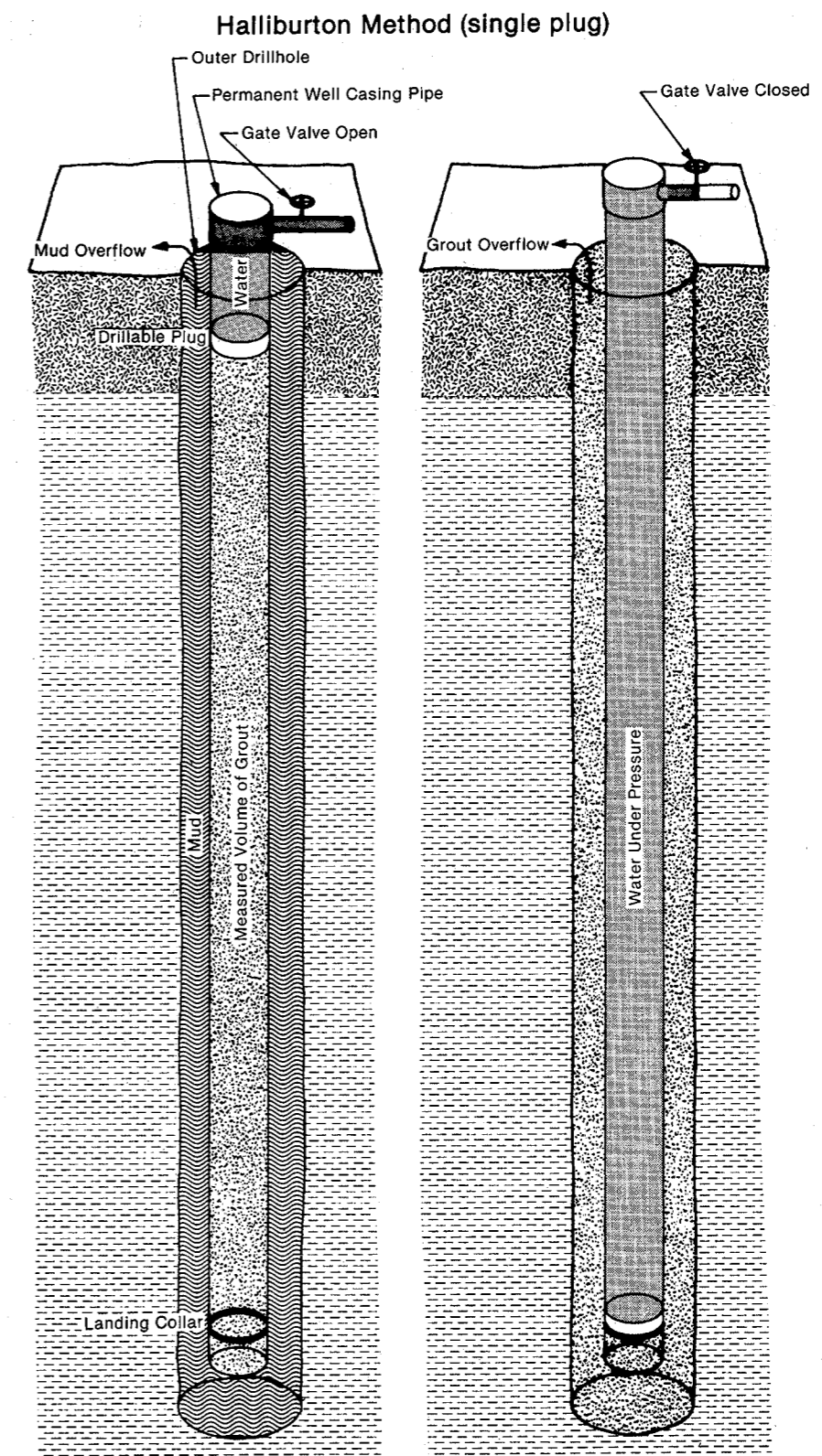
Figure 16. Halliburton (single plug) method for neat cement grouting.
