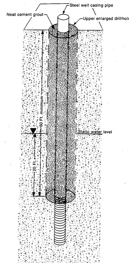
Figure 65. Line G Rotary methods for potable high capacity, school, and wastewater treatment plant wells in unconsolidated aquifers overlain by caving material. The well casing pipe shall extend to the 60-foot depth or 20 feet below the static water level, whichever is greater.
