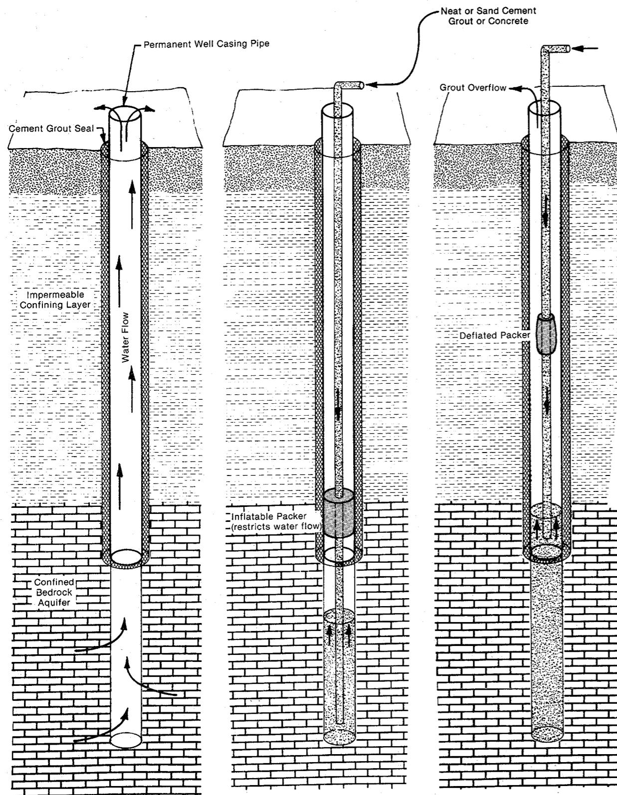
Figure 20. Inflation packer method for permanently abandoning a flowing well.
