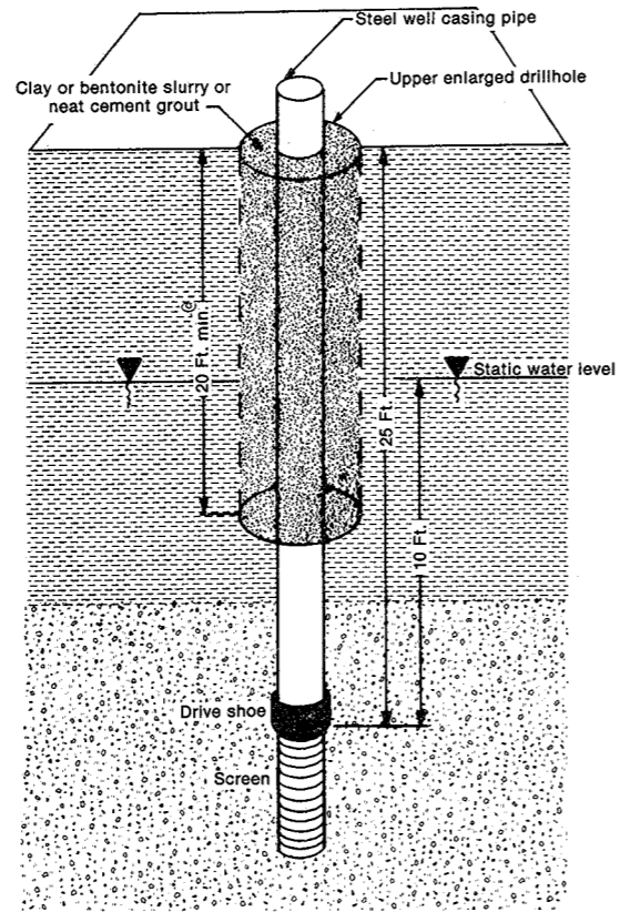
Figure 53. Line B Percussion methods for low capacity* and nonpotable high capacity wells in unconsolidated aquifers overlain by non-caving material. Well casing pipe shall extend to the 25-foot depth or 10 feet below the static water level, whichever is greater.
