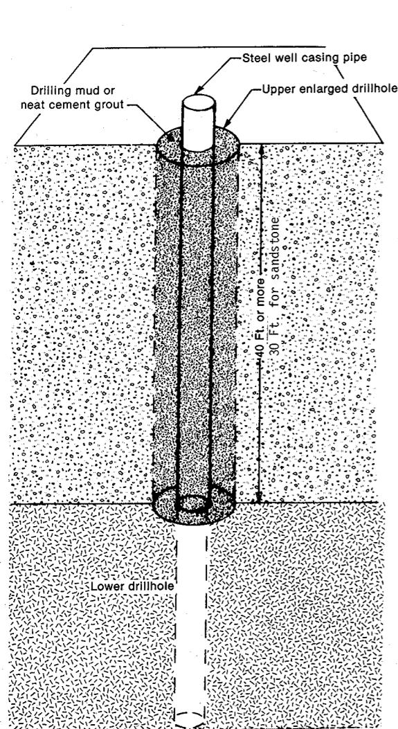
Figure 56. Line C. Rotary methods for low capacity* and nonpotable high capacity wells in all types of bedrock with at least 40 feet of overlying caving material.
