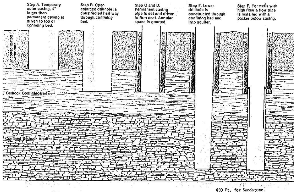
Figure 9. (c) I. Percussion method for flowing well construction—confined bedrock aquifer more than 40 feet below the ground surface with a bedrock confining bed.
