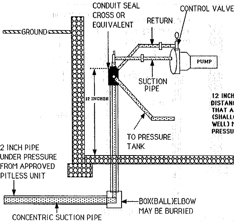
Figure 36c. Alternate offset pump installation discharge piping using a buried box (ball) elbow and seal cross fitting. Figure prepared by T. Roos.
