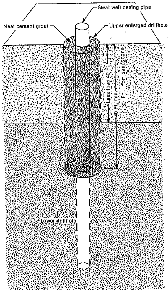
Figure 61. Line B. Rotary methods for low capacity* and nonpotable high capacity wells in all types of bedrock with less than 40 feet of overlying caving material.
