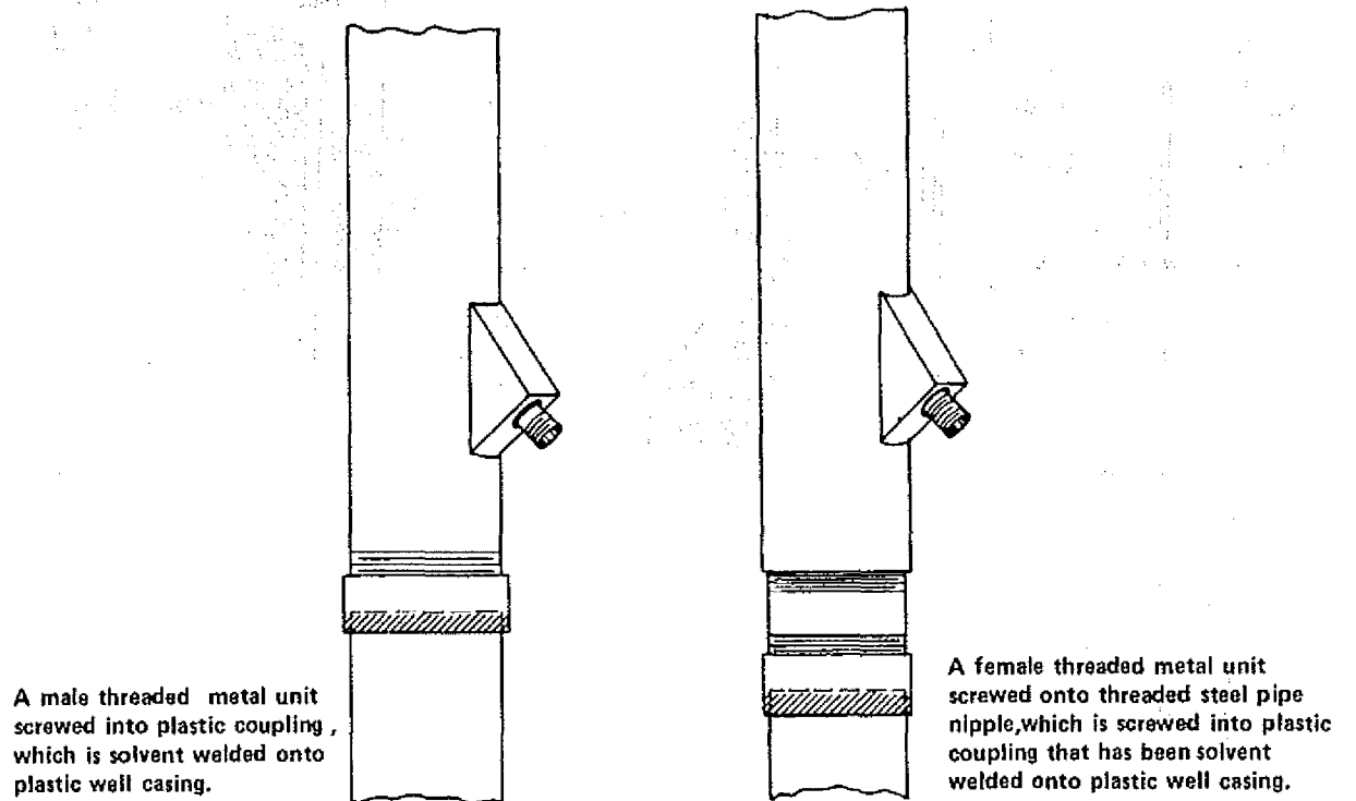
Figure 31. Pitless unit connections for wells with thermoplastic well casing pipe.
