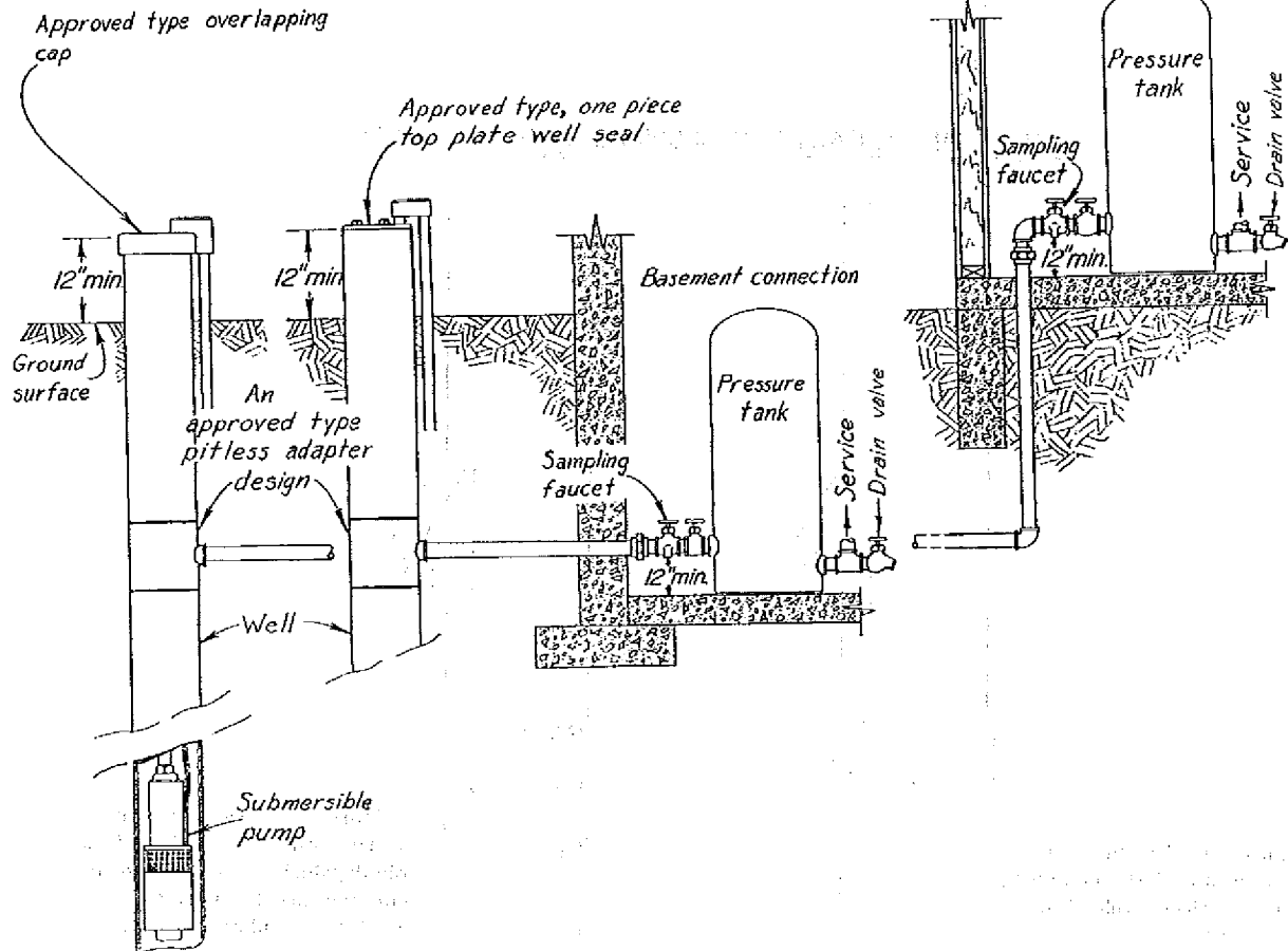
Figure 33. Pump installations for wells with pitless adapters.
