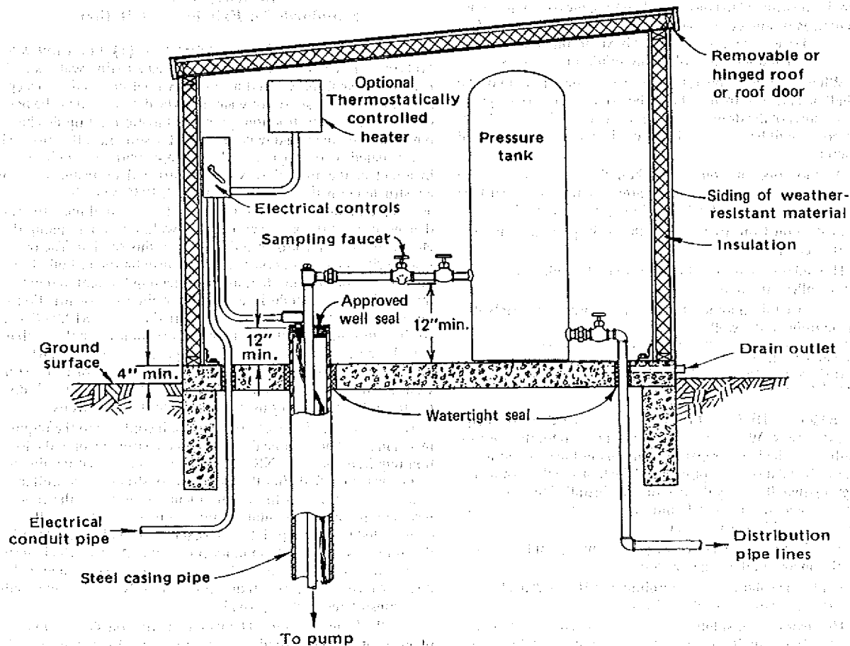
Figure 46. Pumphouse specifications.
