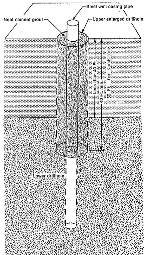
Figure 62. Line B. Rotary methods for low capacity* and nonpotable high capacity wells in all types of bedrock with less than 40 feet of overlying non-caving material.
