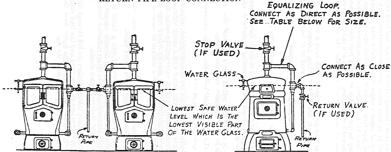
Fig. 1 RETURN PIPE LOOP CONNECTION
