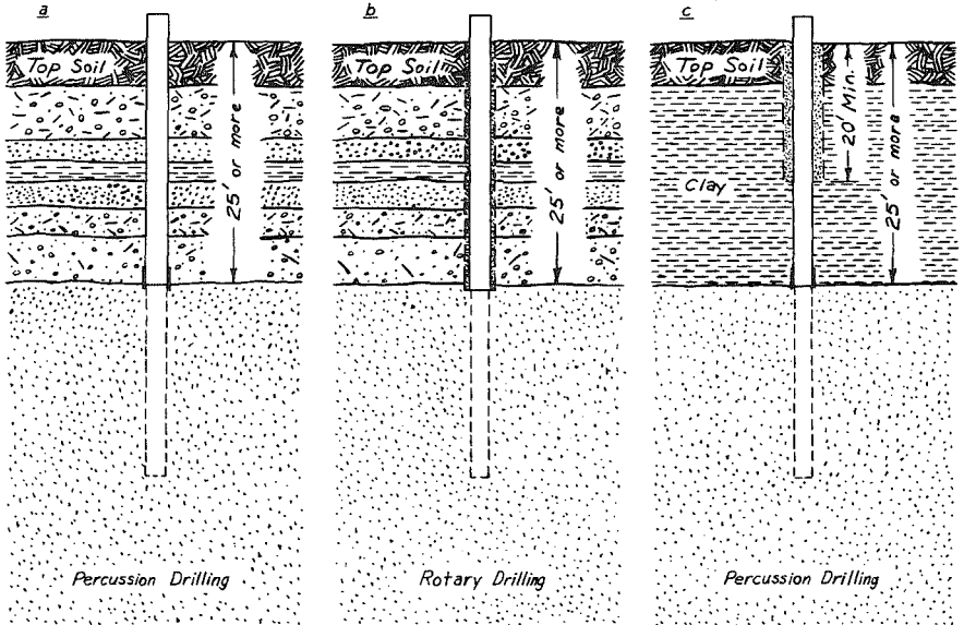
Figure A-21. Construction of Wells Terminating in Sandstone Underlying Unconsolidated Materials comprising mainly Sand and Gravel, or Clay or Similar Material, extending to a depth of 25 feet or greater depth. See Table 1, m and n.
