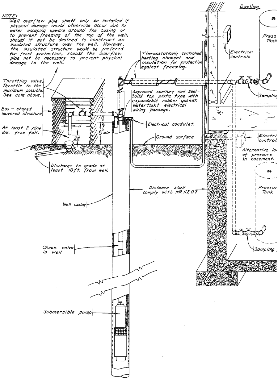
Figure 22. Pump Installation for Flowing Well Using a Submersible Pump and Above-Ground Discharge and Overflow Pipe, if necessary.
