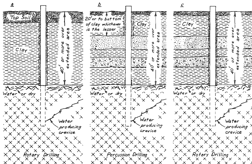
Figure A-18. Construction of Wells Terminating in Granite or Quartzite Underlying Clay or Similar Material or such Materials with some Sand and Gravel Zones, extending to a depth of 40 feet or greater depth. See Table 1, k.
