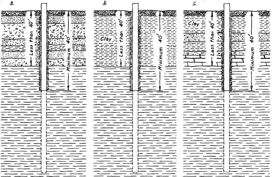
Figure A-15. Construction of Wells Terminating in Shale Underlying Unconsolidated Materials comprising mainly Sand and Gravel, or Clay or Similar Material, or a Mixture of Sand, Gravel and Clay or Similar Material, extending to a depth of less than 40 feet, by either Percussion or Rotary Equipment. See Table 1, i.
