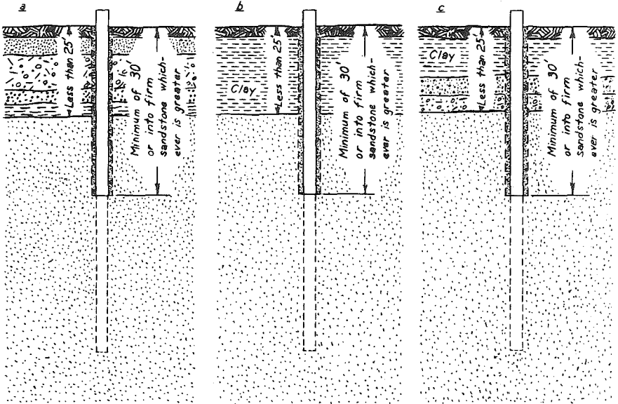
Figure A-23. Construction of Wells Terminating in Sandstone Underlying any Material except Limestone, extending to a depth of less than 25 feet, by either Percussion or Rotary Equipment. See Table 1, o.
