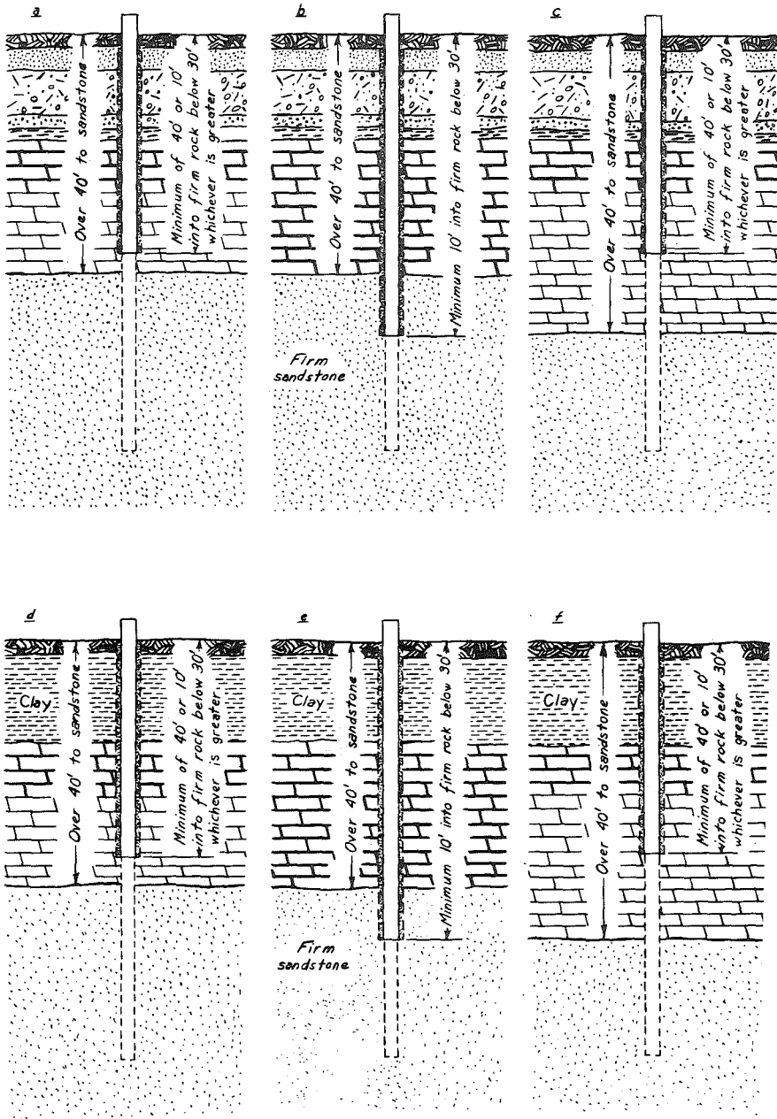
Figure A-25. Construction of Wells Terminating in Sandstone Underlying Limestone extending to a depth greater than 40 feet with or without Unconsolidated Overburden over the Limestone, by either Percussion or Rotary Equipment. See Table 1, q.
