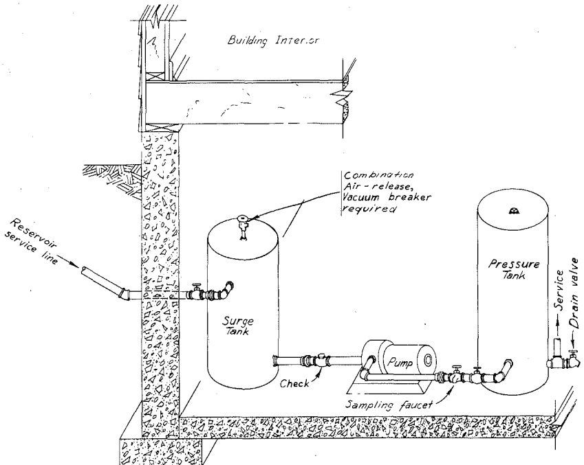
Figure 17. Acceptable Installation of Booster Pump on Service Line from Reservoir, when necessary.
