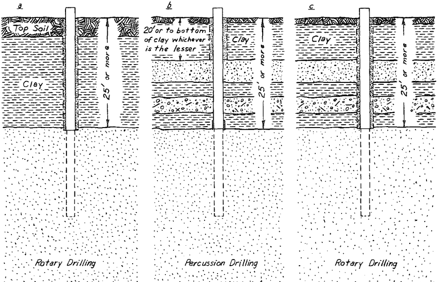
Figure A-22. Construction of Wells Terminating in Sandstone Underlying Clay or Similar Material or such Materials with some Sand and Gravel, extending to a depth of 25 feet or greater depth. See Table 1, n.
