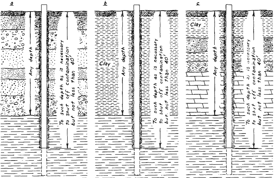
Figure A-16. Construction of Wells Terminating in Shale Underlying Unconsolidated Materials comprising mainly Sand and Gravel, or Clay or Similar Material, or a Mixture of Sand, Gravel and Clay or Similar Material, extending to variable depths, by either Percussion or Rotary Equipment. See Table 1, g, h and i.
