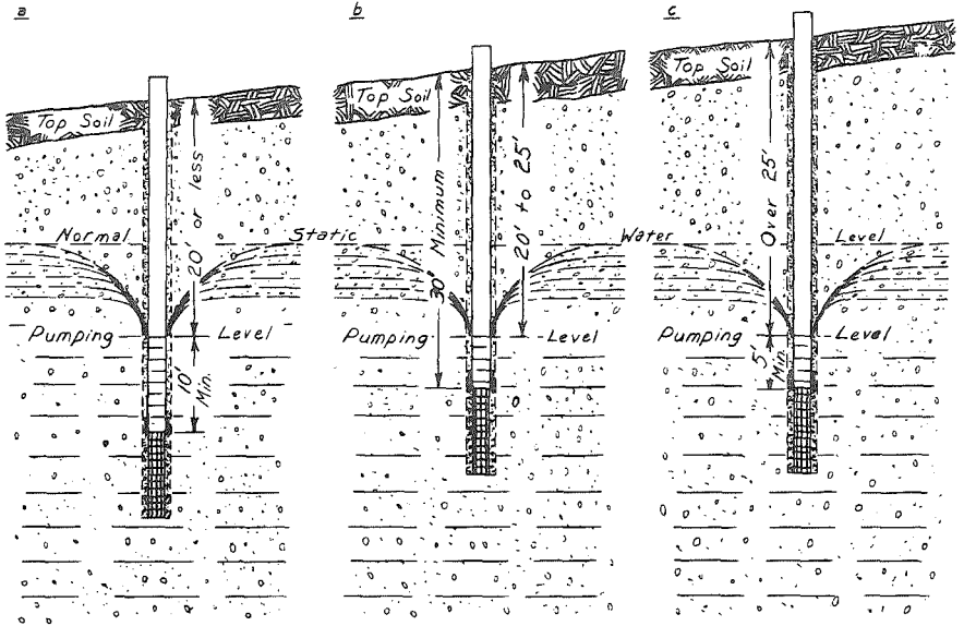
Figure A-3. Construction of Wells in Sand and Gravel with Screens, by Rotary Equipment. See Table 1, a.
