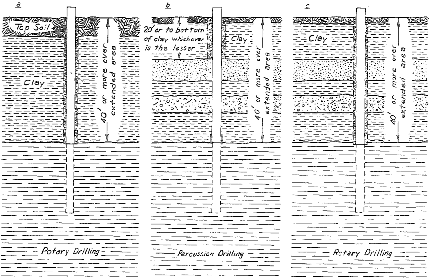
Figure A-14. Construction of Wells Terminating in Shale Underlying Clay or Similar Material or such materials with some Sand and Gravel Zones, extending to a depth of 40 feet or greater depth. See Table I, h.
