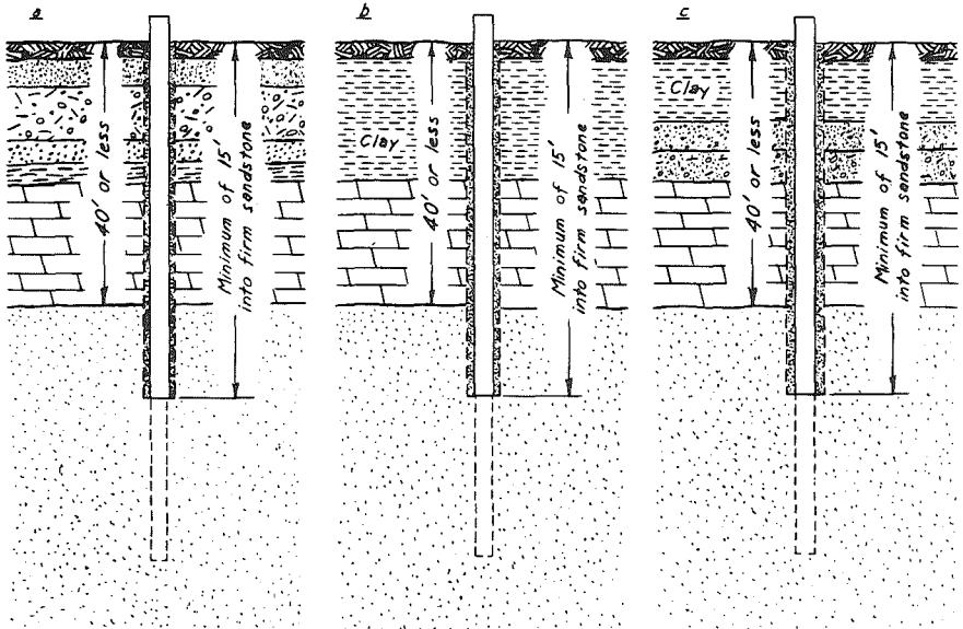
Figure A-24. Construction of Wells Terminating in Sandstone Underlying Limestone extending to a depth of 40 feet or less with or without Unconsolidated Overburden over the Limestone, by either Percussion or Rotary Equipment. See Table 1, p.
