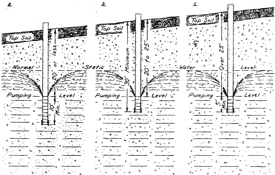
Figure A-2. Construction of Wells in Sand and Gravel without Screens, by Percussion Equipment. See Table 1, a.
