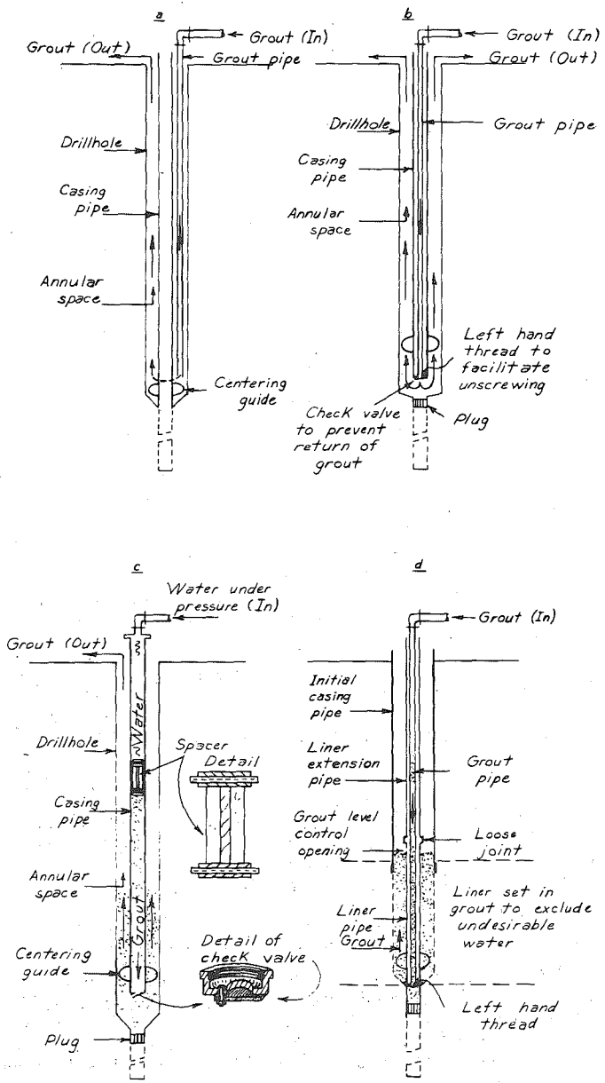
Figure 25. Arrangements for Grouting Annular Space.
