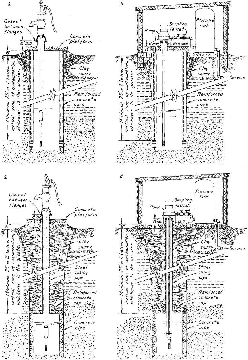
Figure 5. Sanitary Construction of Dug Type Wells and Acceptable Methods of Installation of Pumps. See NR 112.11.
