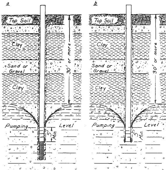
Figure A-6. Construction of Wells Terminating in Sand and Gravel Underlying Clay or Similar Material containing layers of Sand and Gravel, with and without Screens, by Rotary Equipment. See Table 1, b.
