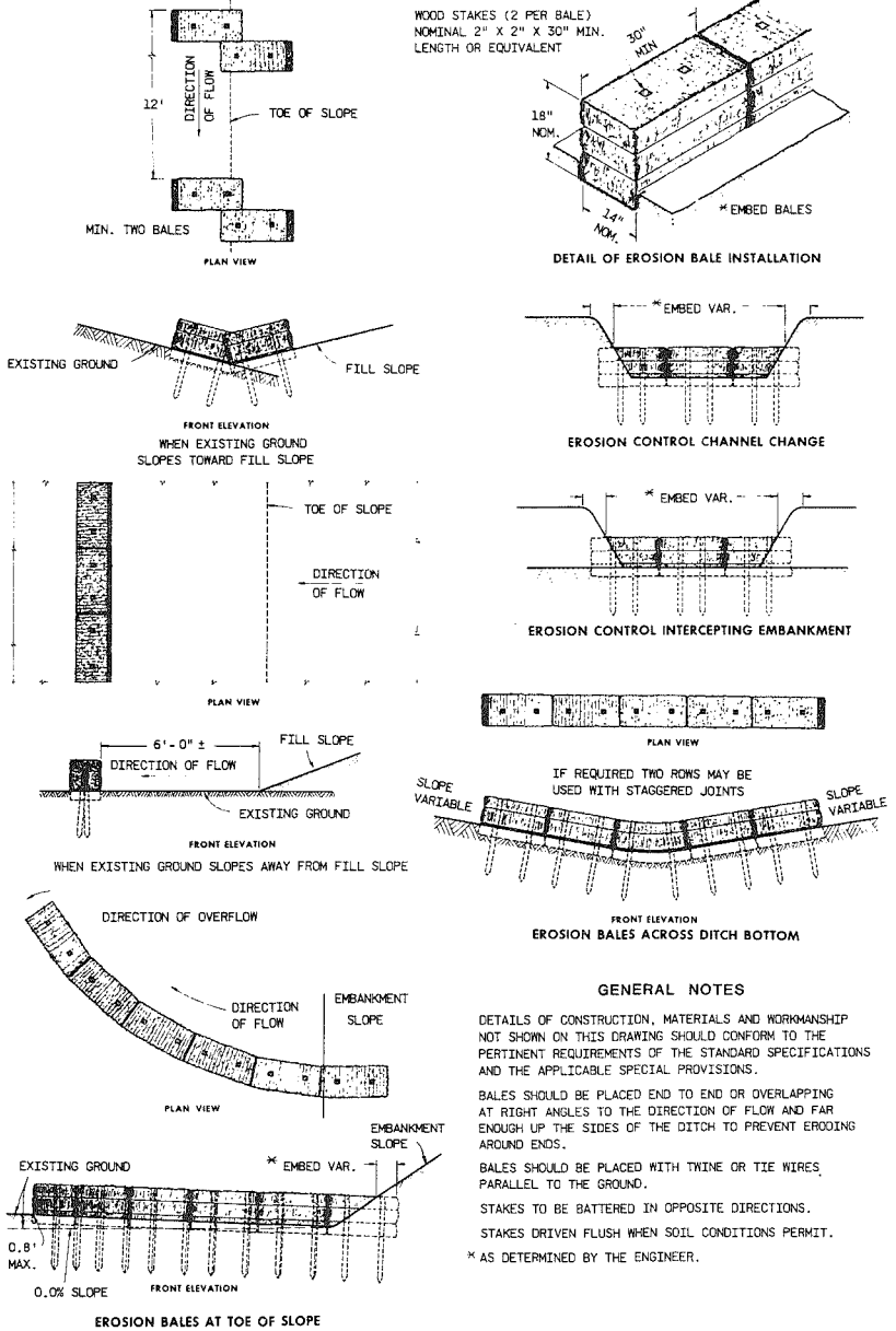
PLACEMENT OF EROSION BALES FIGURE 4
