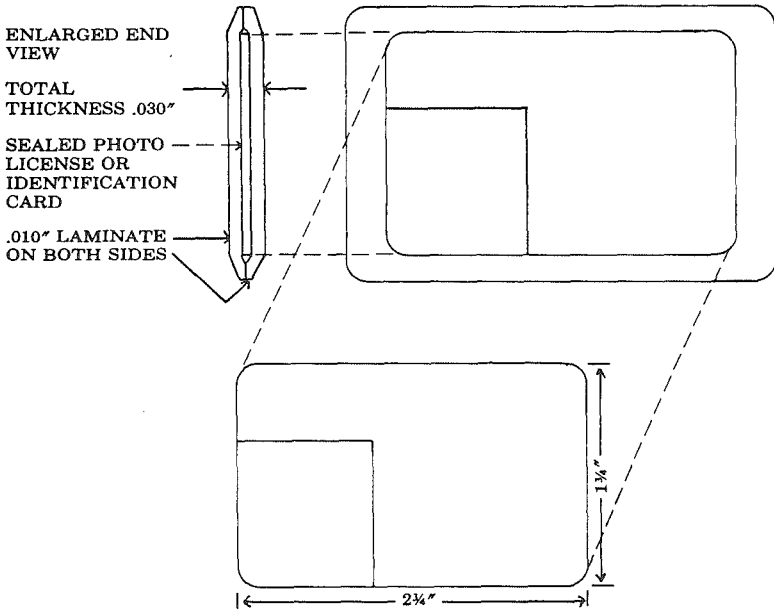
FIGURE 3 Laminate Specifications
