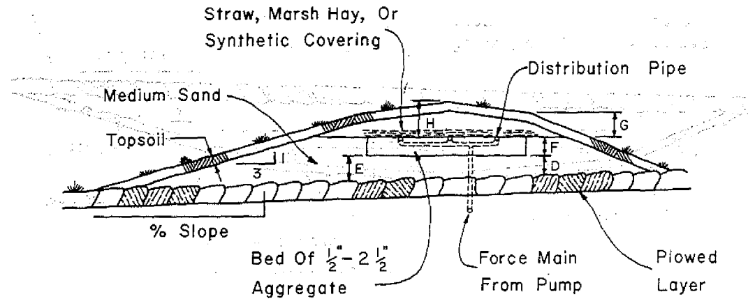
Cross Section Of A Mound System Using A Bed For The Absorption Area
