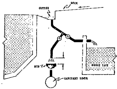
deck drainage to gutter system
