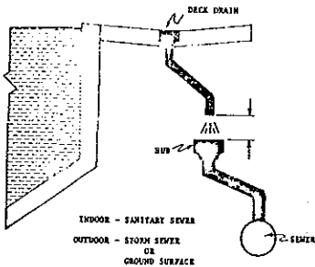
deck drainage
