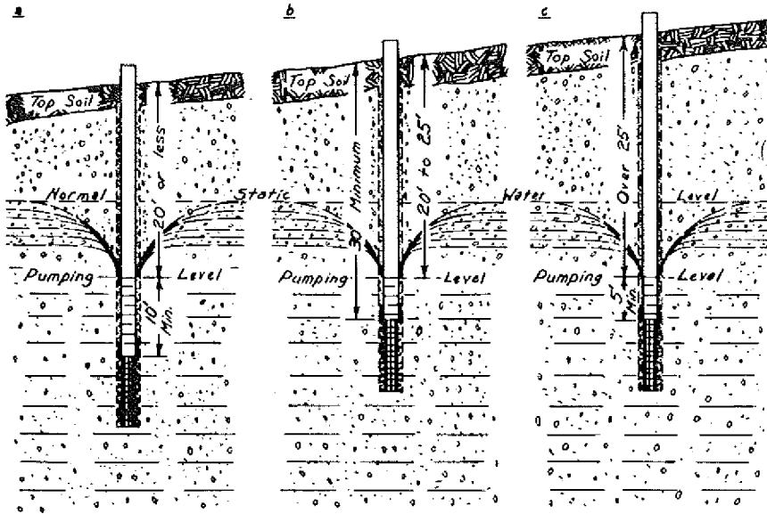
Figure A-3. Construction of Wells in Sand and Gravel with Screens, by Rotary Equipment. See Table I, a.
