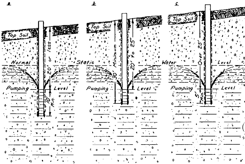
Figure A-4. Construction of Wells in Sand and Gravel without Screens, by Rotary Equipment. See Table I, a.
