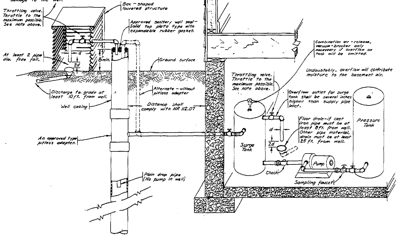
Figure 24. Pump Installation for Flowing Well Showing alternatives of Above-Ground Discharge or Approved Pitless Adapter Installation with a Surge Tank and Booster Pump and Overflow Options at the Surge Tank or Top of the Well, if either is necessary.
