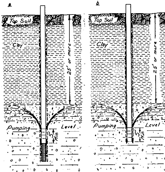
Figure A-8. Construction of Wells Terminating in Sand and Gravel Underlying Clay or Similar Material, with and without Screens, by Rotary Equipment. See Table I, c.
