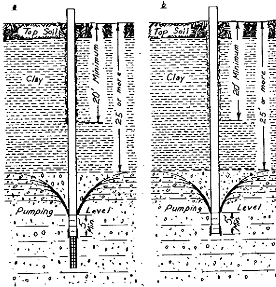
Figure A-7. Construction of Wells Terminating in Sand and Gravel Underlying Clay or Similar Material, with and without Screens, by Percussion Equipment. See Table I, c.
