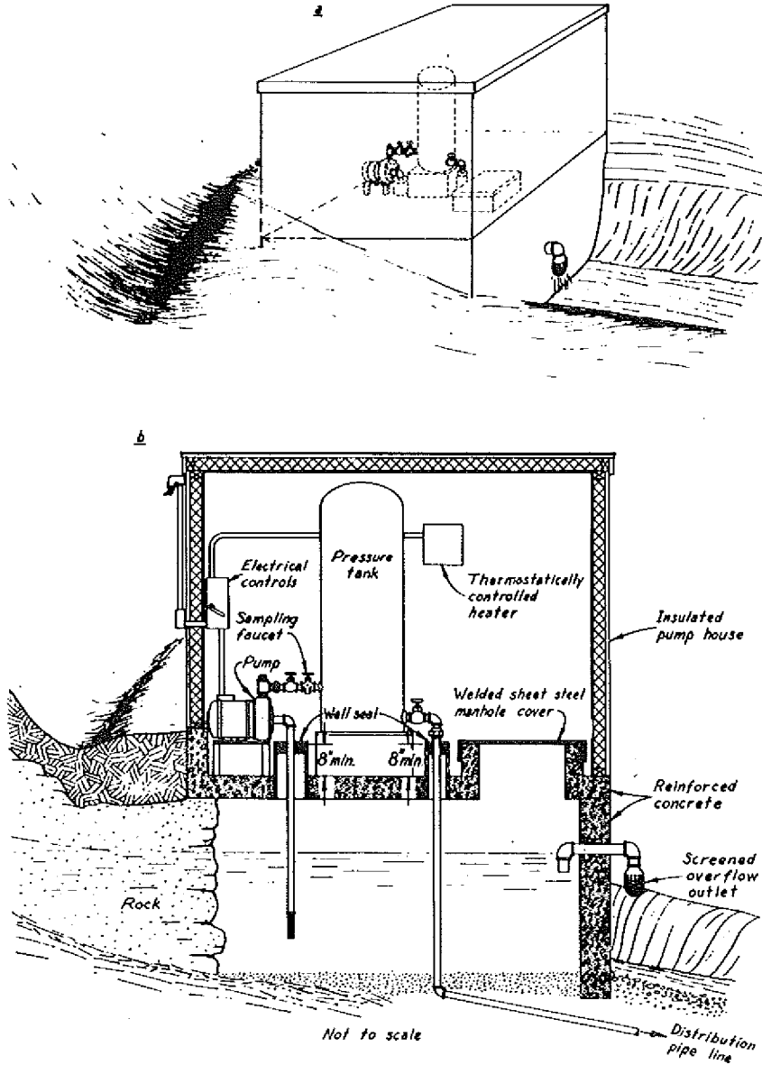
Figure 7. Spring House.
