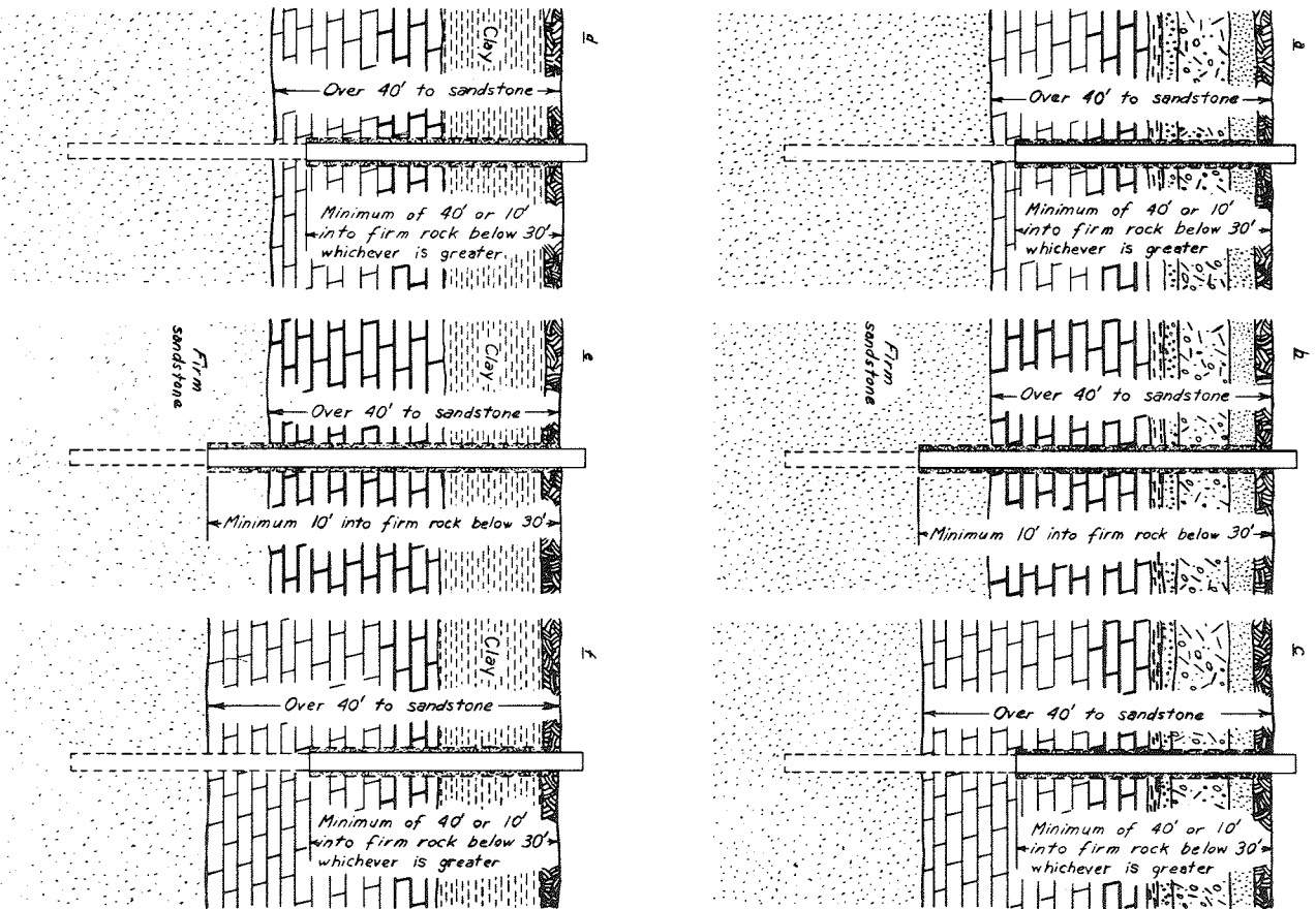
Figure A-25. Construction of Wells Terminating in Sandstone Underlying Limestone extending to a depth greater than 40 feet with or without Unconsolidated Overburden over the Limestone, by either Percussion or Rotary Equipment. See Table I, 9.
