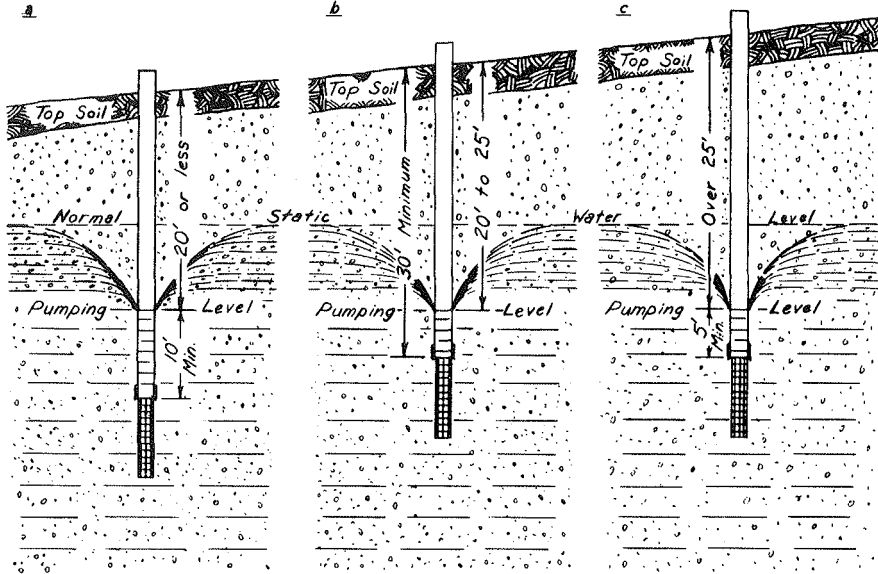
Figure A-1. Construction of Wells in Sand and Gravel with Screens, by Percussion Equipment. See Table 1, a.
