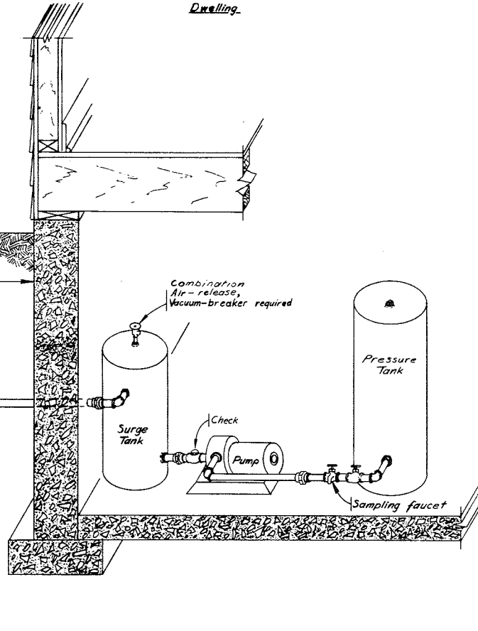
Figure 19. Pump Installation for Flowing Artesian Well using an Approved Pitless Adapter, Surge Tank and Booster Pump with no Overflow Provision.
