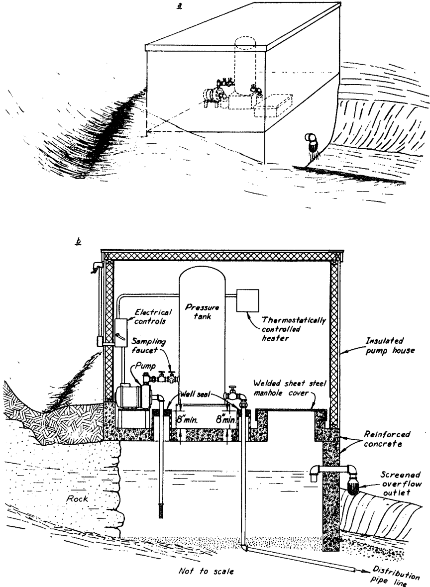
Figure 7. Spring House.
