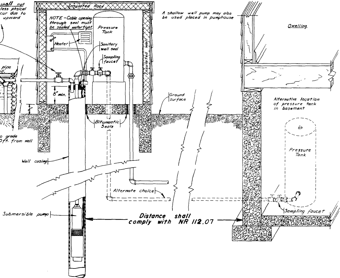
Figure 20. Pump Installation for Flowing Well using Submersible Pump and Above-Ground Discharge and Overflow Provision, if necessary.
