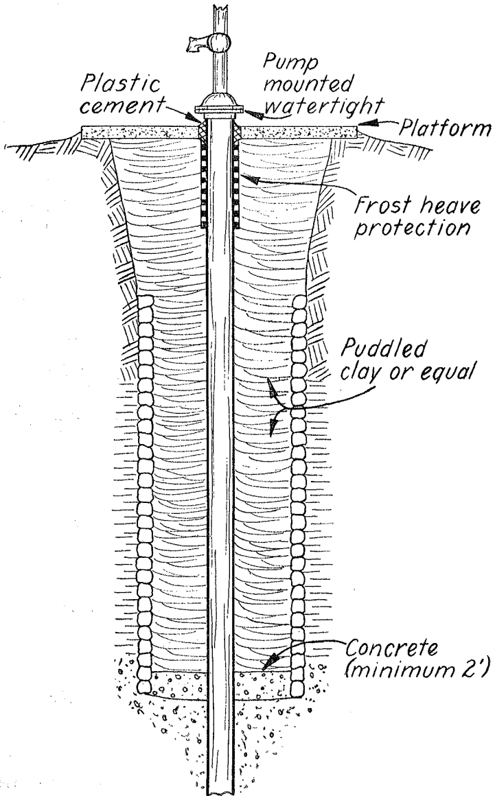
Figure 9. Drilled Well Constructed in Existing Dug Well. See Wis. Adm. Code section RD 12.05 (7).
