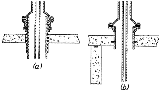
Figure 10. Hand Pump Mountings. (a) On well casing pipe through a water-tight pump flange. (b) On a section of pipe set in concrete well top and fitted with a pipe flange. See RD 12.09 (1) and (2) (a).
