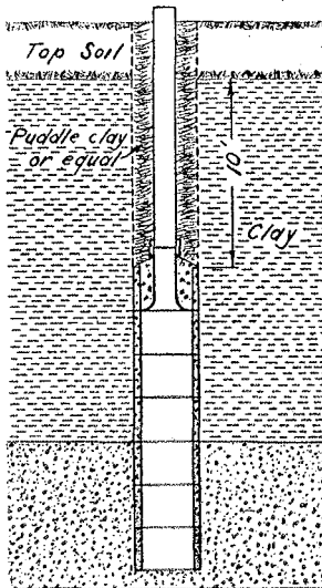
Figure 6. Bored Type Well Construction. See Wis. Adm. Code section RD 12.05 (4).
