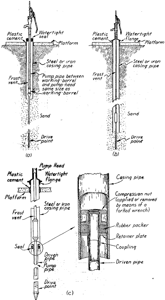
Figure 7. Driven Point Well Construction. Illustration (c) shows suitable method of returning frost drain water to well when impervious soil is present. See Wis. Adm. Code section RD 12.05 (5).
