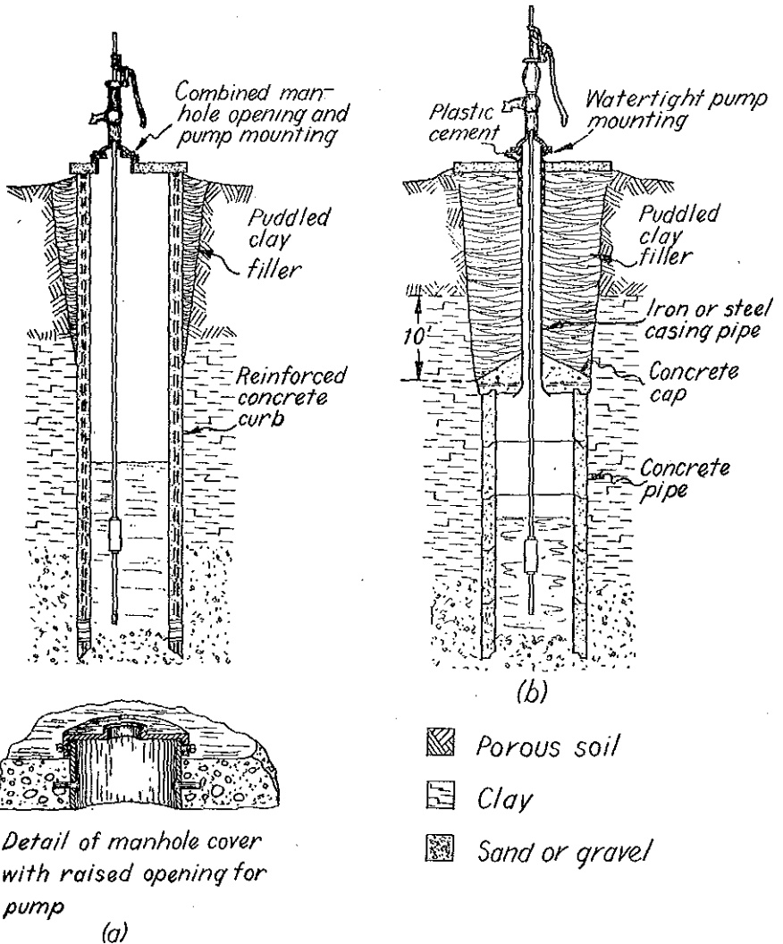
Figure 8. Sanitary Construction of Dug Wells. See H 55.05 (6).
