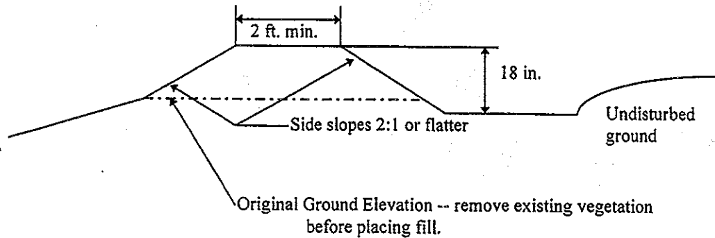
FIG. E-10. TEMPORARY DIVERSION
