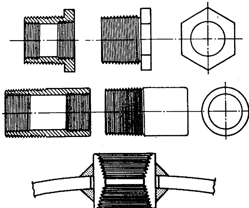
FIG. PG-59.1 TYPICAL BOILER BUSHINGS
