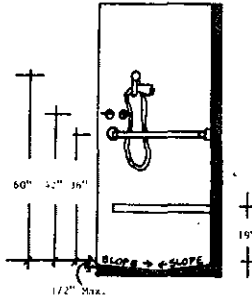
Section View - Shower
