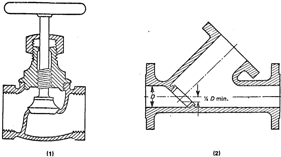
FIG. 122.1.7(C) TYPICAL GLOBE VALVES
