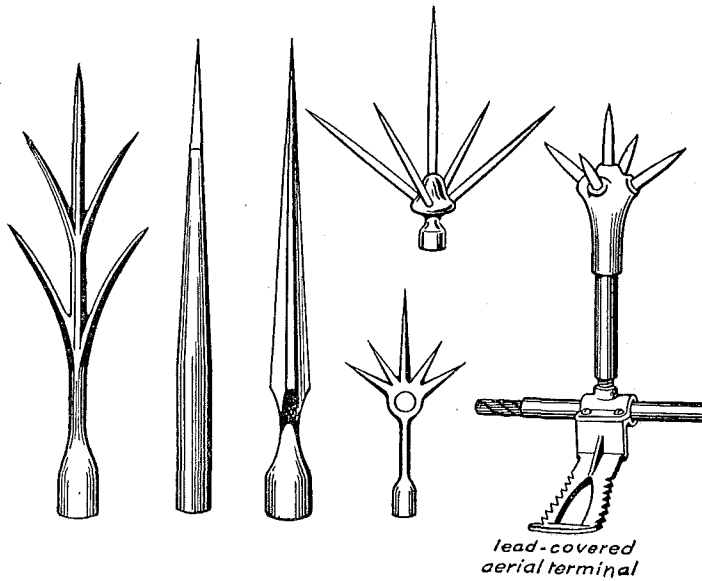
Air Terminals
