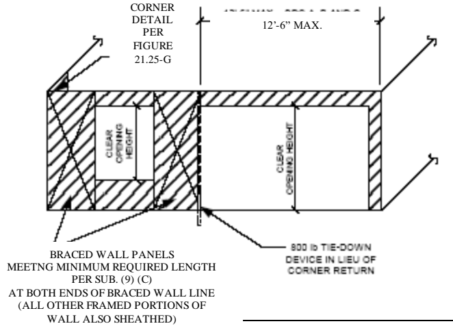
FIGURE 21.25-J CONTINUOUSLY SHEATHED BRACED WALL LINE – FIRST BRACED WALL PANEL AWAY FROM END OF WALL LINE WITH TIE DOWN
